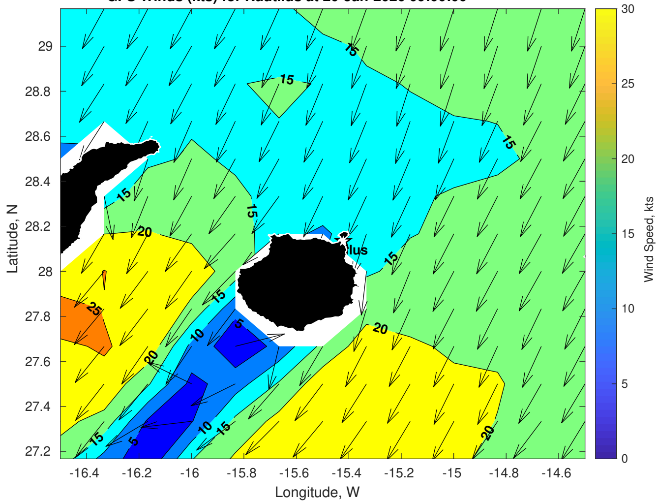
GFS Winds (kts) for Nautilus at 20-Jan-2026 09:00:00
