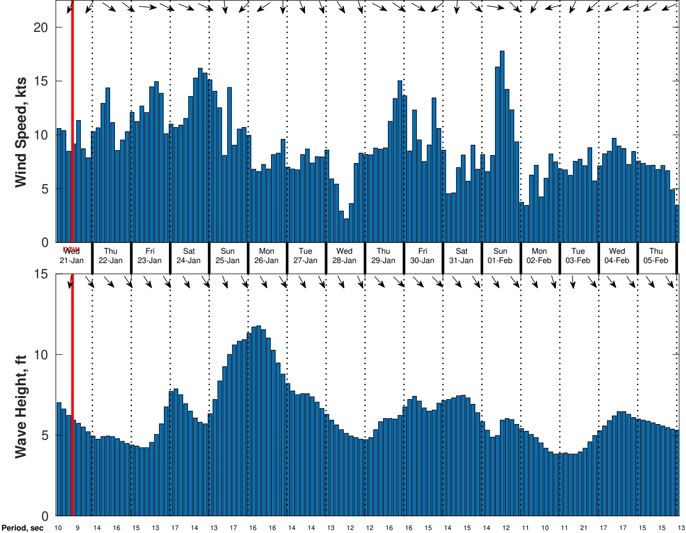
Wind & Wave Forecast for Nautilus from 20-Jan-2026 02:00:00 to 05-Feb-2026 02:00:00
