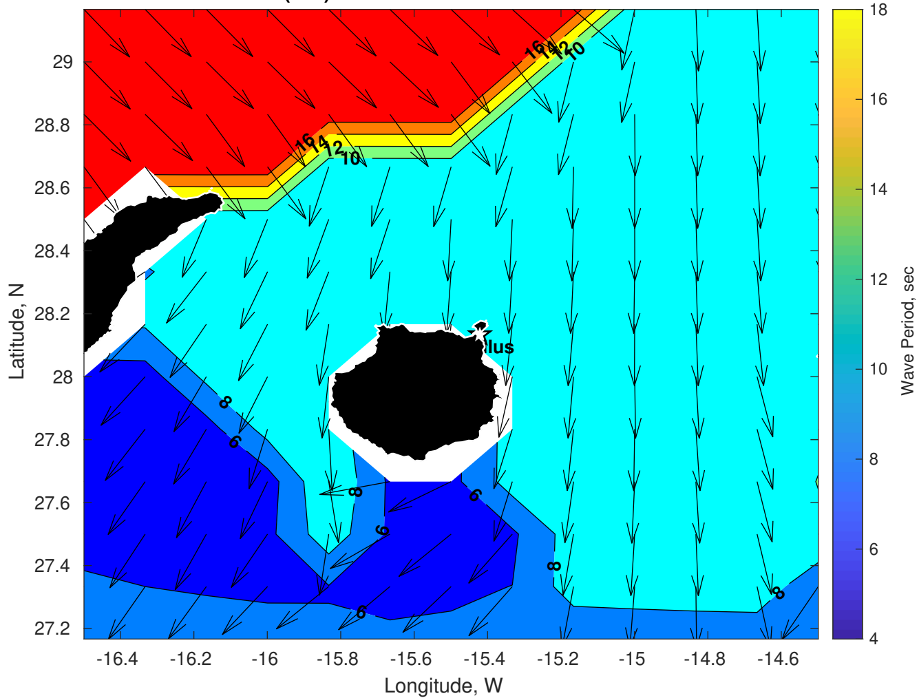
GFS Wave Period (sec) for Nautilus at 20-Jan-2026 09:00:00
