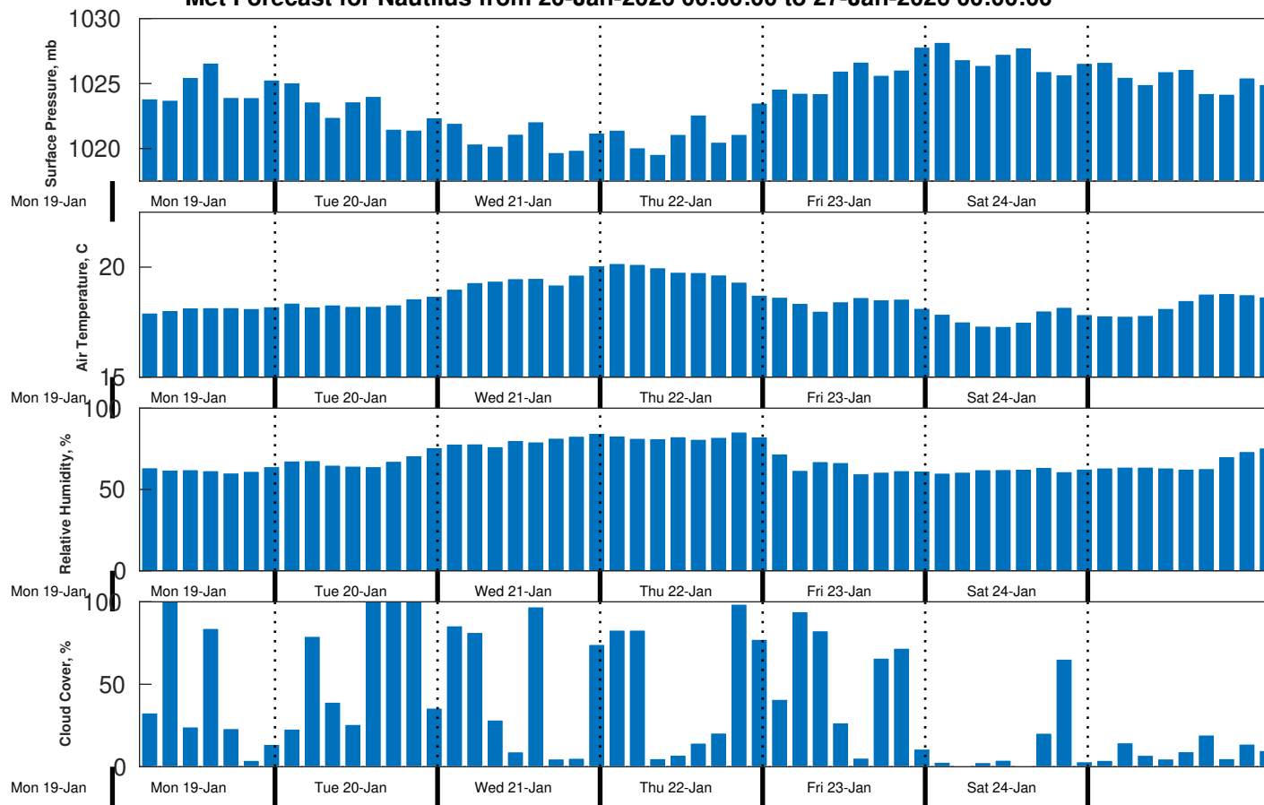
Met Forecast for Nautilus from 20-Jan-2026 00:00:00 to 27-Jan-2026 00:00:00
