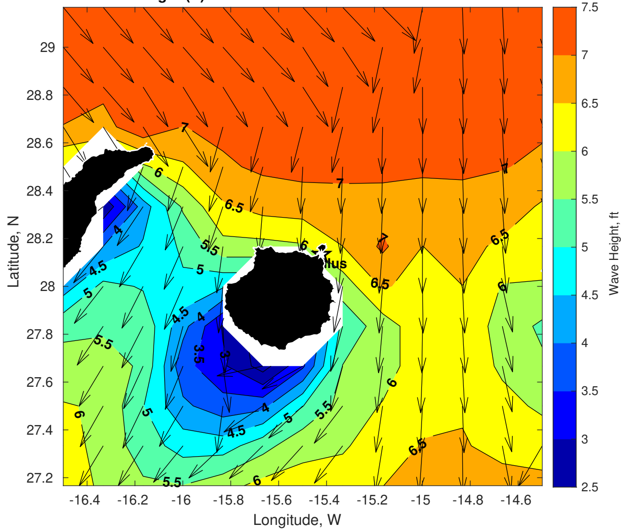
GFS Wave Height (ft) for Nautilus at 20-Jan-2026 09:00:00
