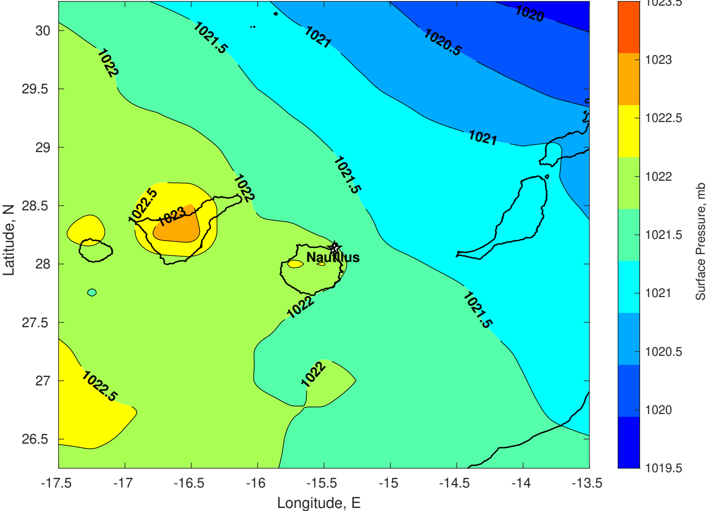
Surface Pressure (mb) for Nautilus at 22-Jan-2026 00:00:00
