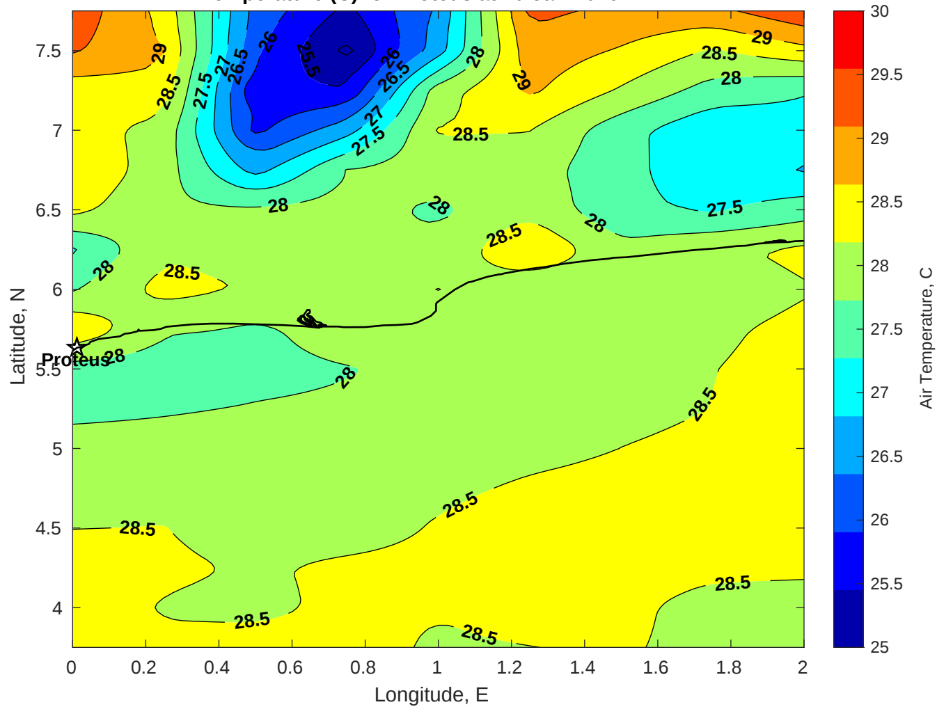
Air Temperature (C) for Proteus at 20-Jan-2026
