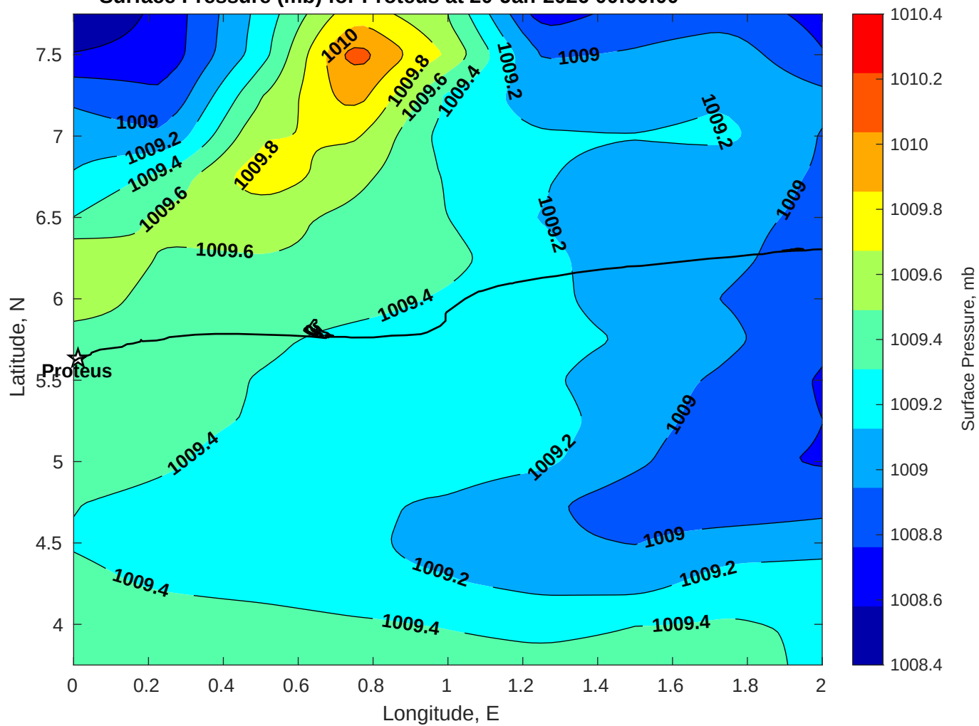
Surface Pressure (mb) for Proteus at 20-Jan-2026 00:00:00
