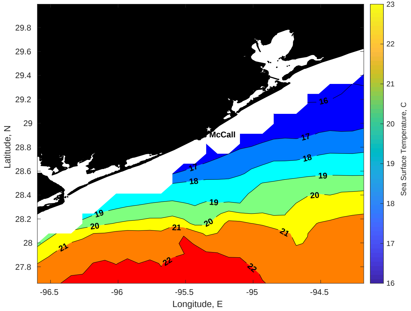
SST for Brooks McCall at 20-Jan-2026 00:00:00
