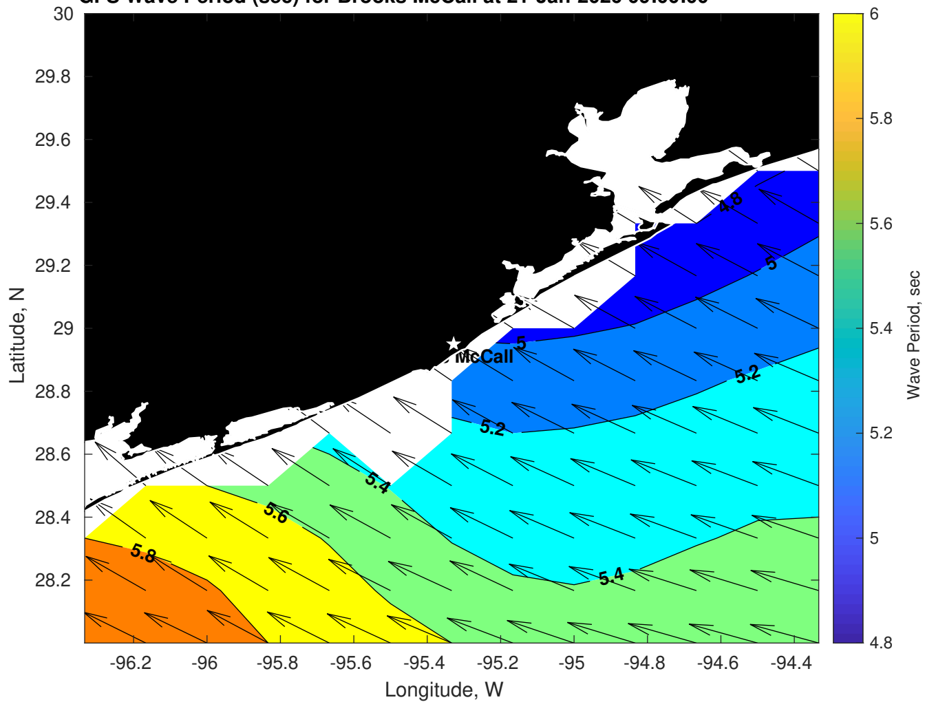
GFS Wave Period (sec) for Brooks McCall at 21-Jan-2026 09:00:00
