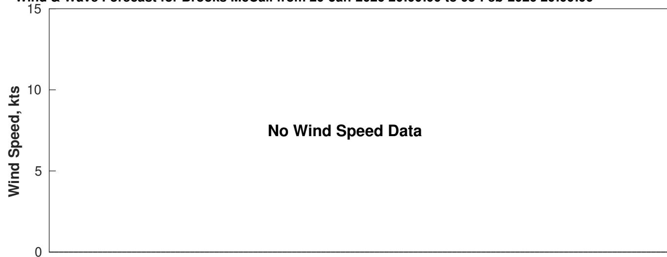
Wind & Wave Forecast for Brooks McCall from 20-Jan-2026 20:00:00 to 05-Feb-2026 20:00:00
