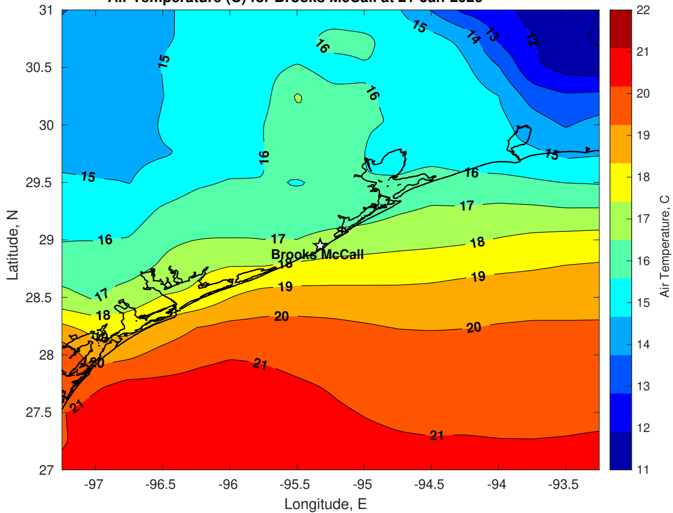
Air Temperature (C) for Brooks McCall at 21-Jan-2026
