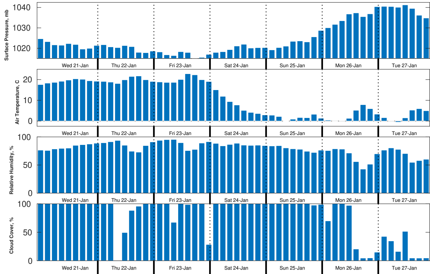
Met Forecast for Brooks McCall from 21-Jan-2026 00:00:00 to 28-Jan-2026 00:00:00
