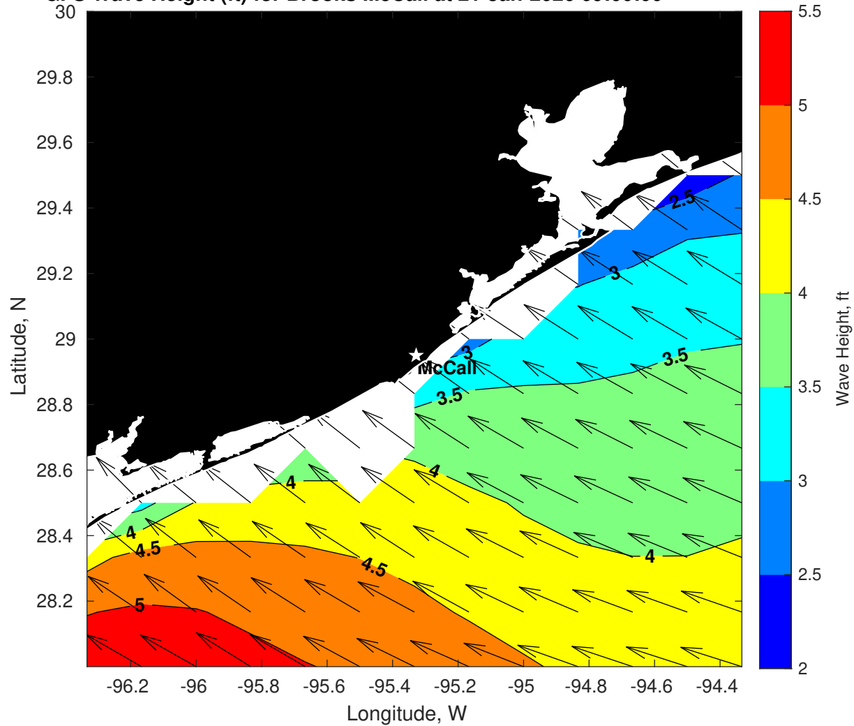
GFS Wave Height (ft) for Brooks McCall at 21-Jan-2026 09:00:00
