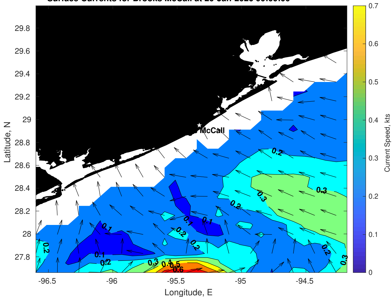
Surface Currents for Brooks McCall at 20-Jan-2026 00:00:00
