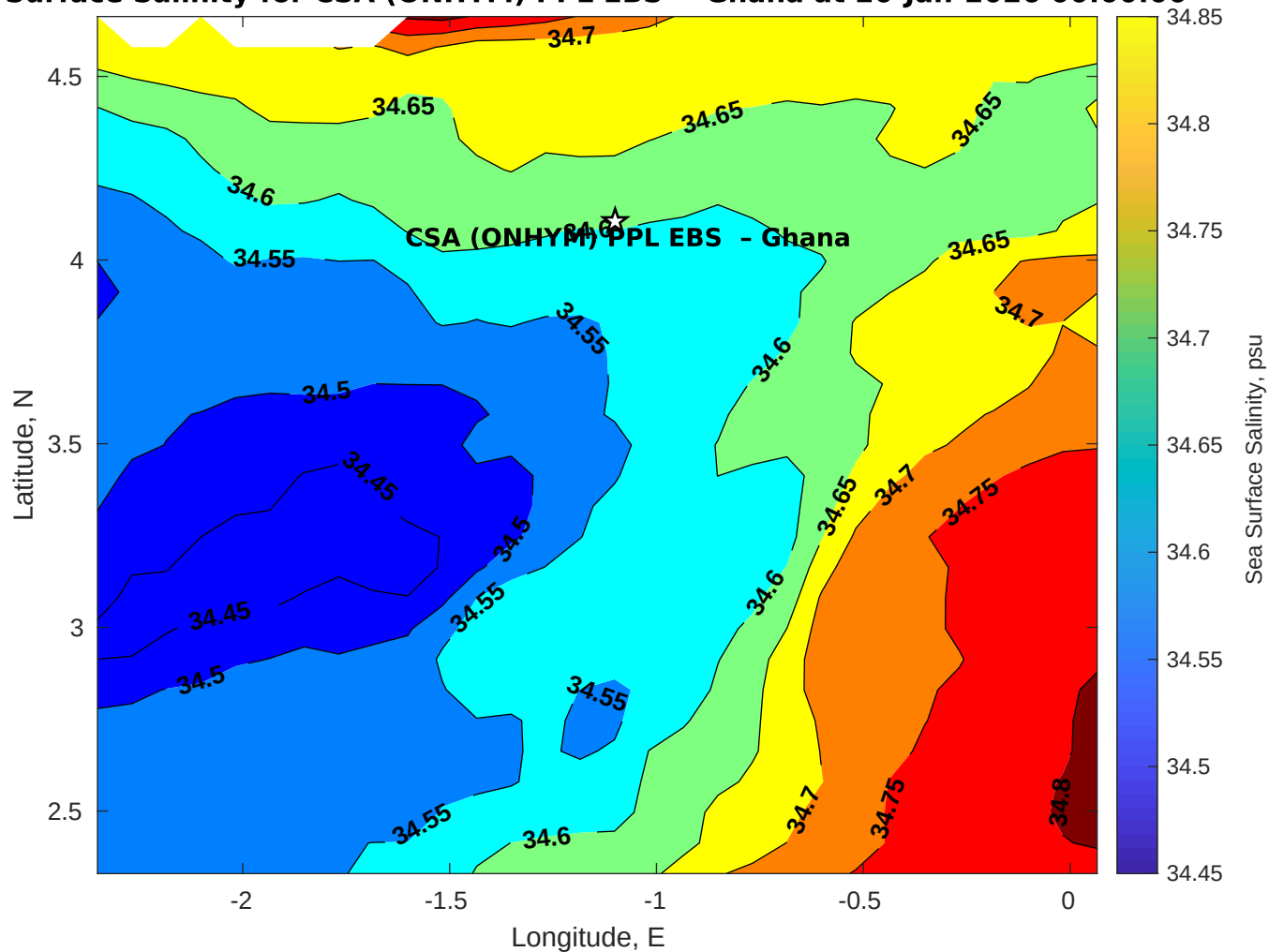
Surface Salinity for CSA (ONHYM) PPL EBS - Ghana at 20-Jan-2026 00:00:00
