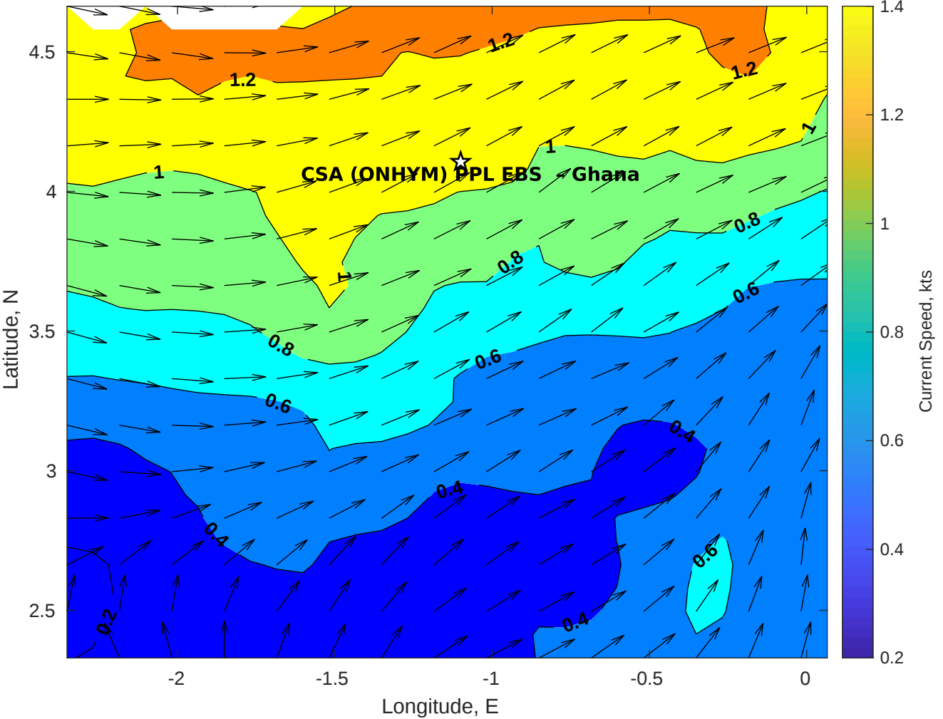
Surface Currents for CSA (ONHYM) PPL EBS - Ghana at 20-Jan-2026 00:00:00
