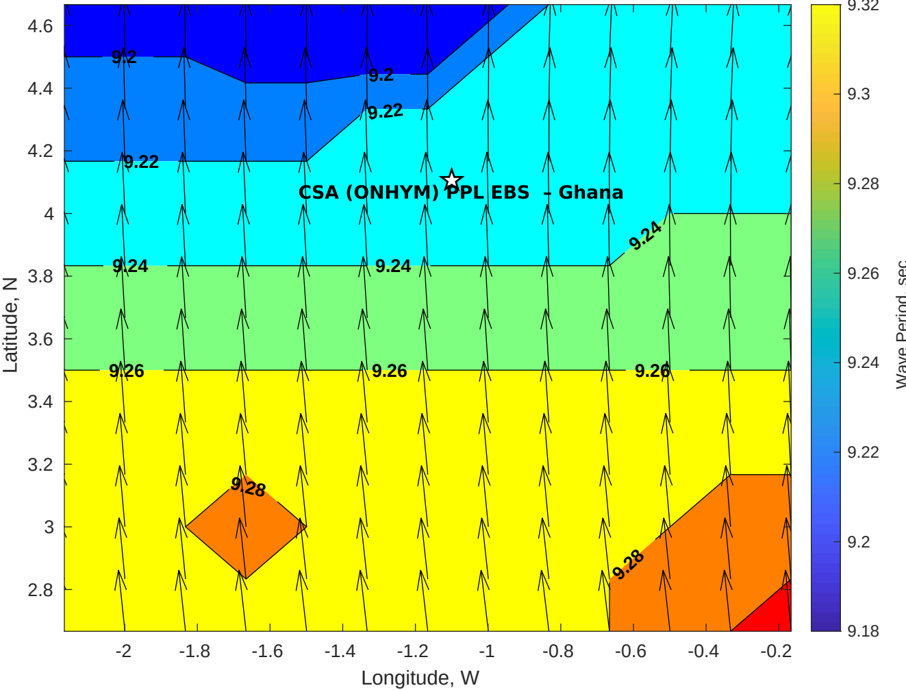
GFS Wave Period (sec) for CSA (ONHYM) PPL EBS - Ghana at 21-Jan-2026 09:00:00
