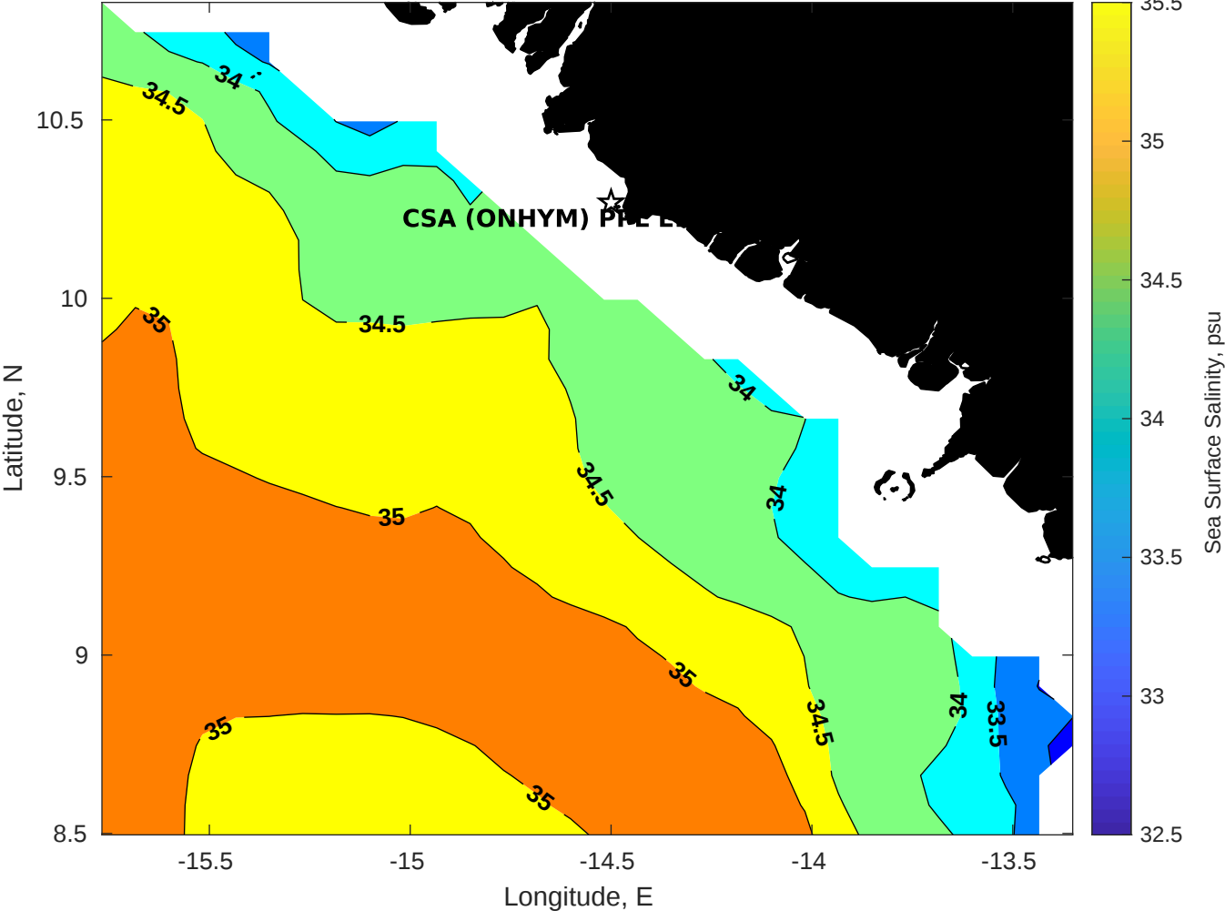
Surface Salinity for CSA (ONHYM) PPL EBS - Guinea at 20-Jan-2026 00:00:00
