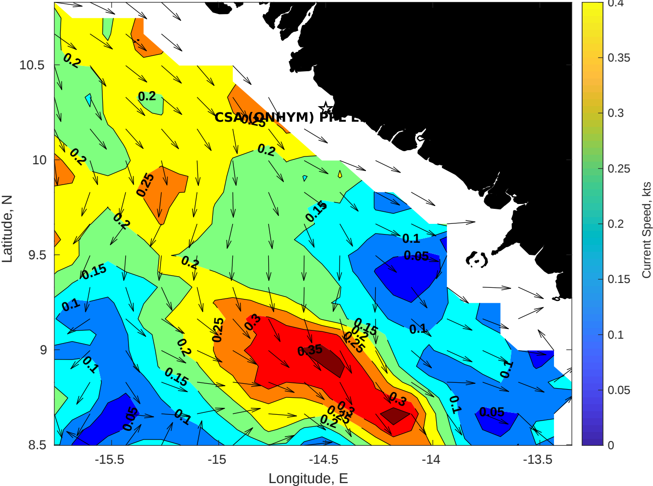
Surface Currents for CSA (ONHYM) PPL EBS - Guinea at 20-Jan-2026 00:00:00
