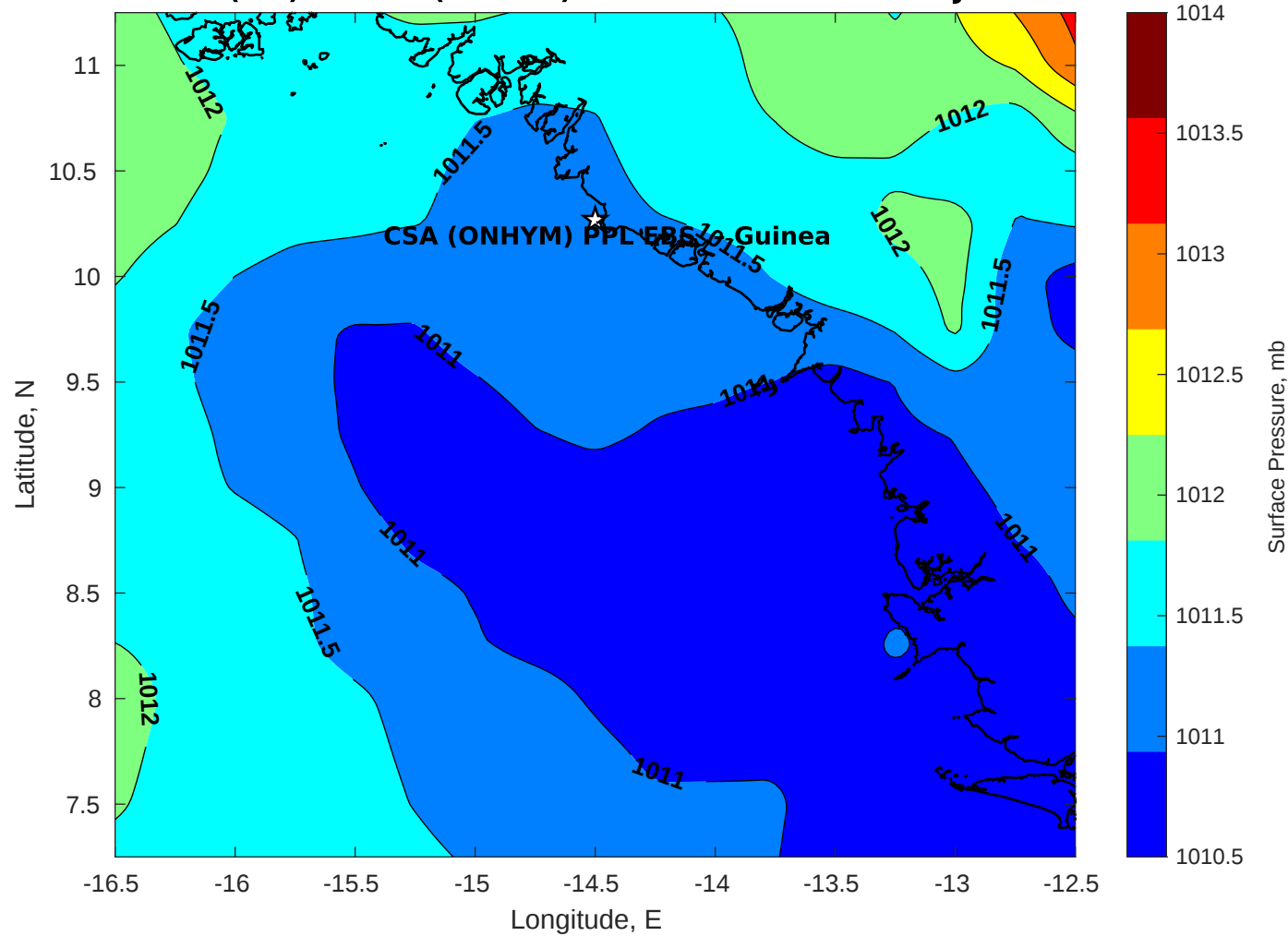
Surface Pressure (mb) for CSA (ONHYM) PPL EBS - Guinea at 23-Jan-2026 00:00:00
