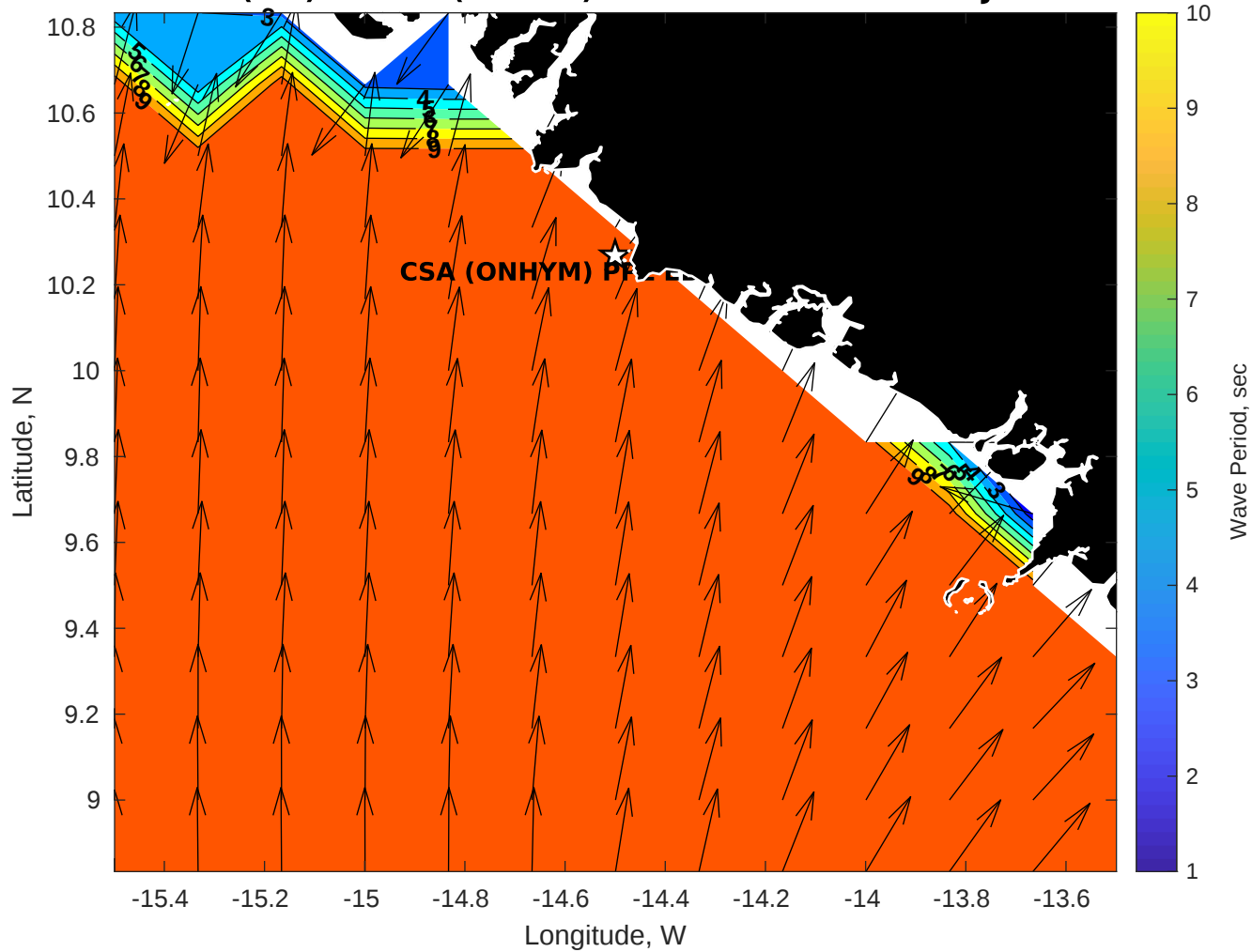
GFS Wave Period (sec) for CSA (ONHYM) PPL EBS - Guinea at 21-Jan-2026 09:00:00
