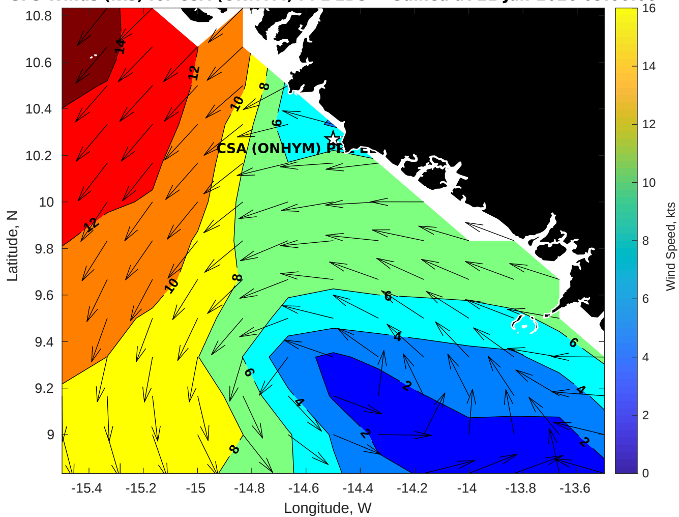
GFS Winds (kts) for CSA (ONHYM) PPL EBS - Guinea at 21-Jan-2026 09:00:00
