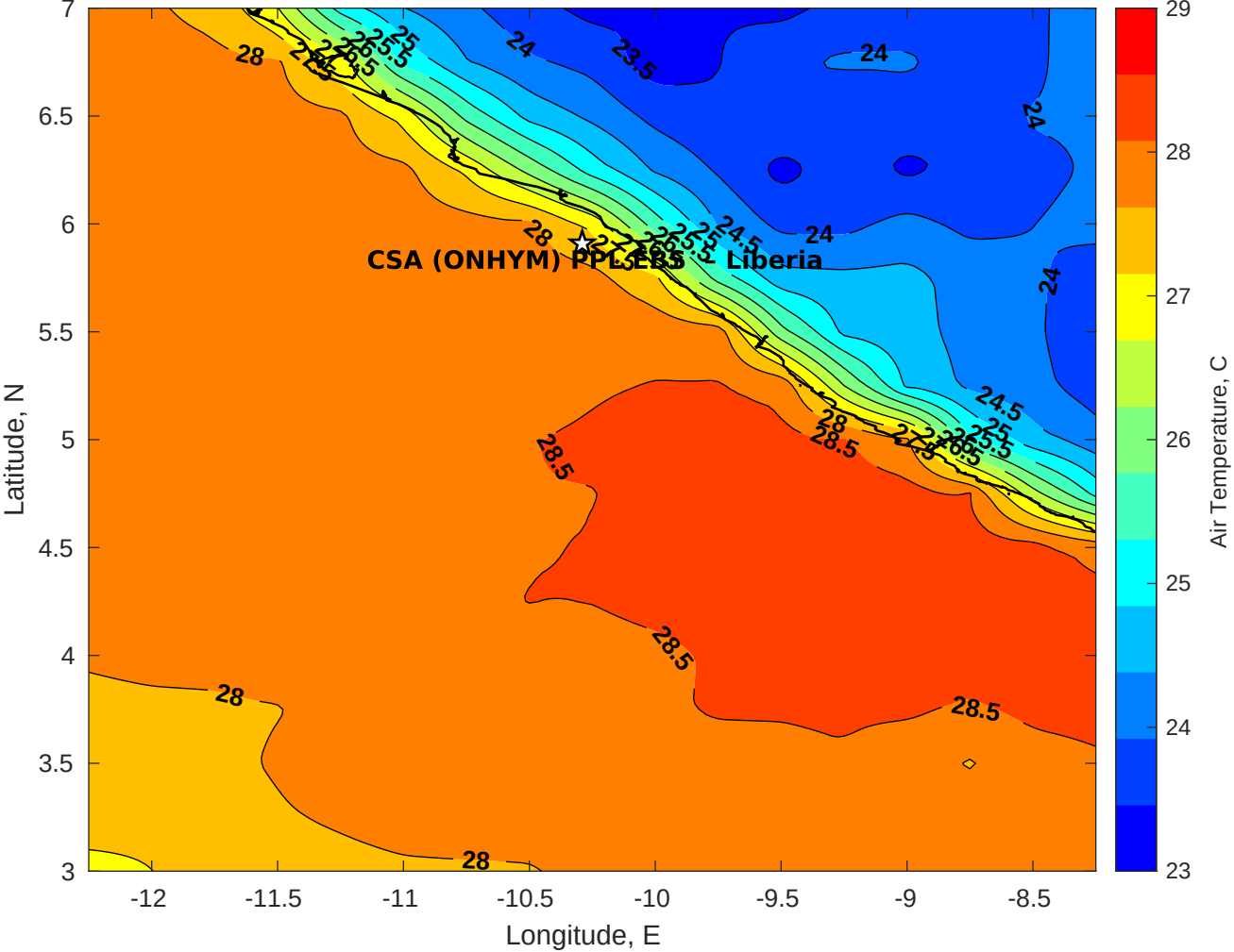
Air Temperature (C) for CSA (ONHYM) PPL EBS - Liberia at 21-Jan-2026
