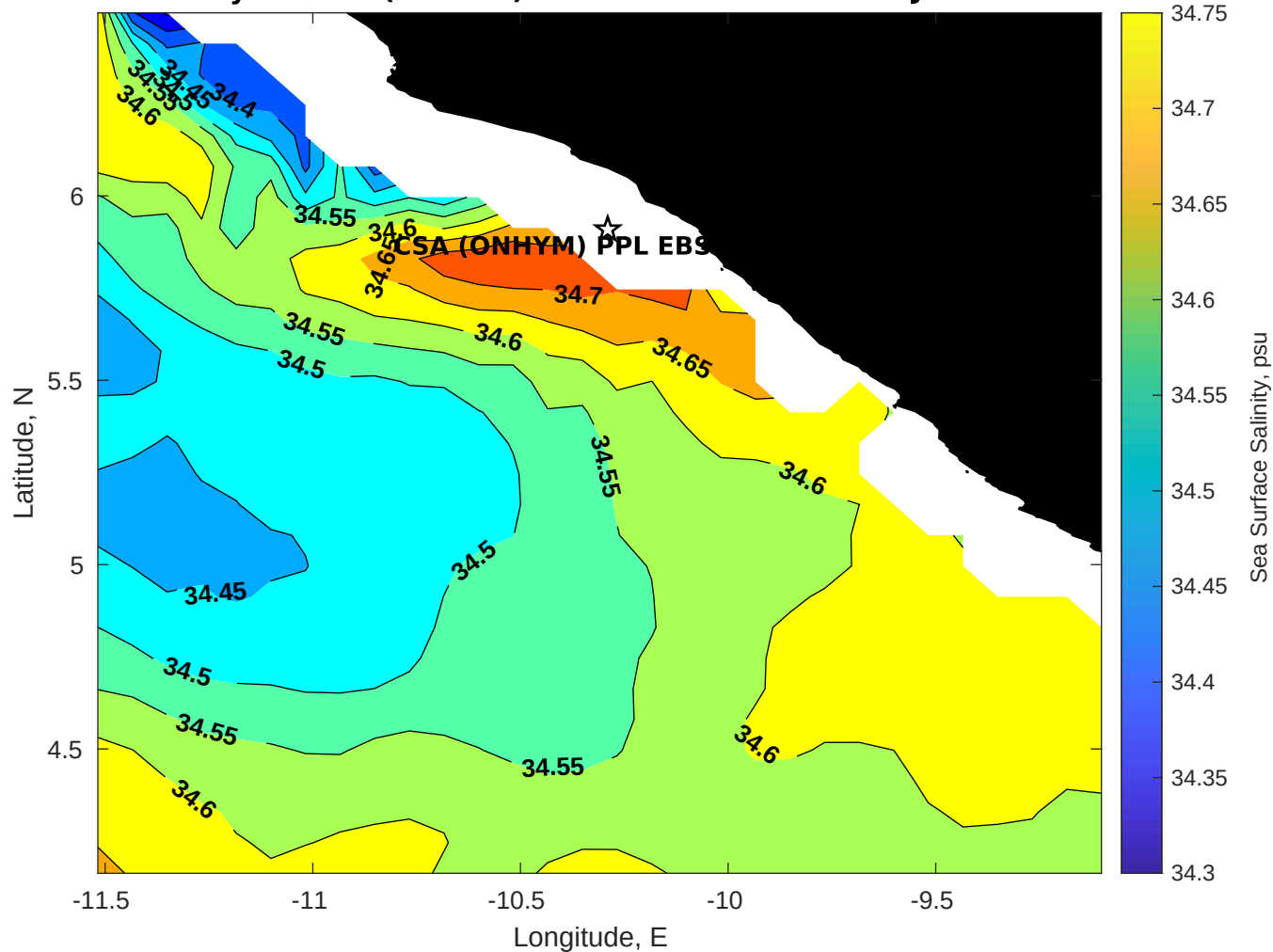
Surface Salinity for CSA (ONHYM) PPL EBS - Liberia at 20-Jan-2026 00:00:00
