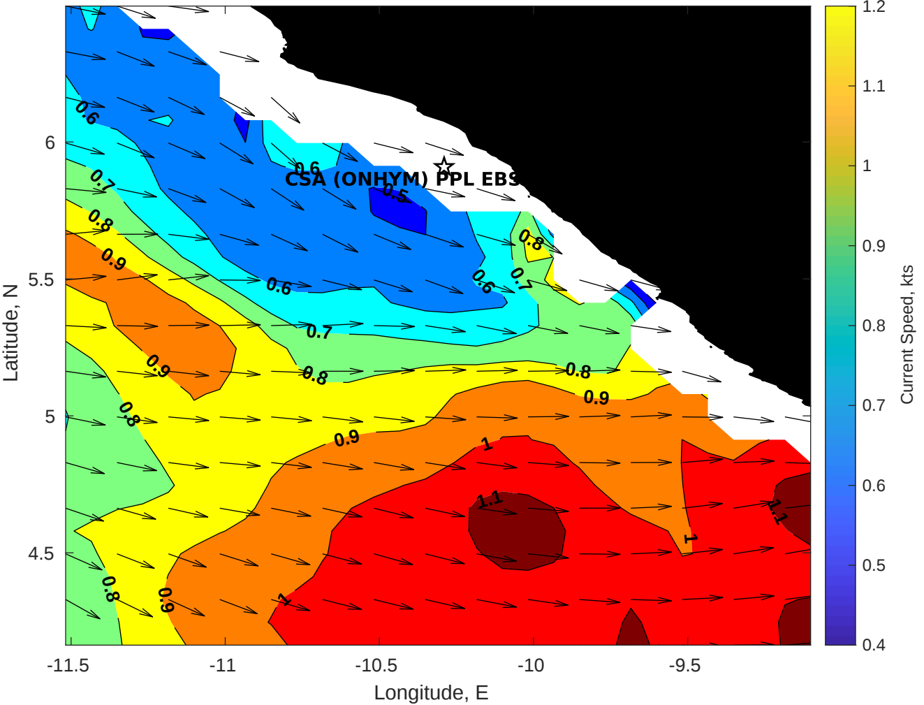
Surface Currents for CSA (ONHYM) PPL EBS - Liberia at 20-Jan-2026 00:00:00
