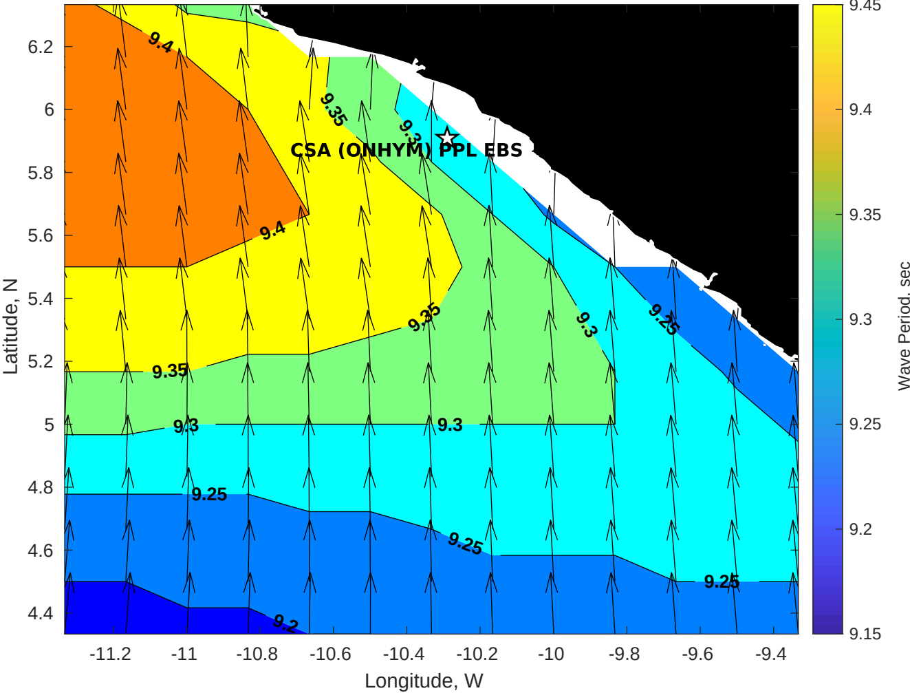
GFS Wave Period (sec) for CSA (ONHYM) PPL EBS - Liberia at 21-Jan-2026 09:00:00
