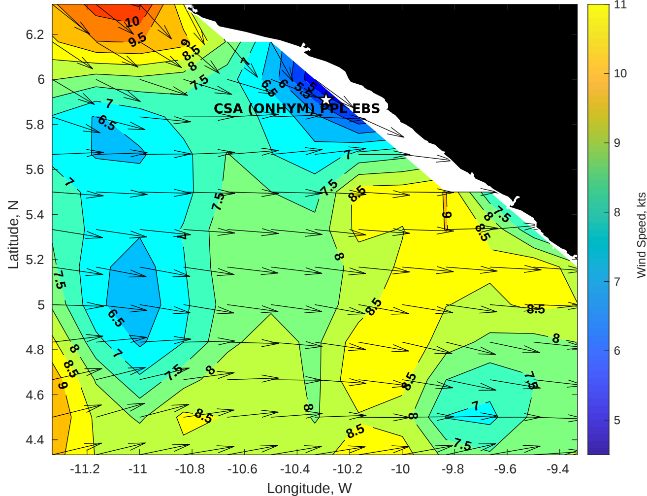
GFS Winds (kts) for CSA (ONHYM) PPL EBS - Liberia at 21-Jan-2026 09:00:00
