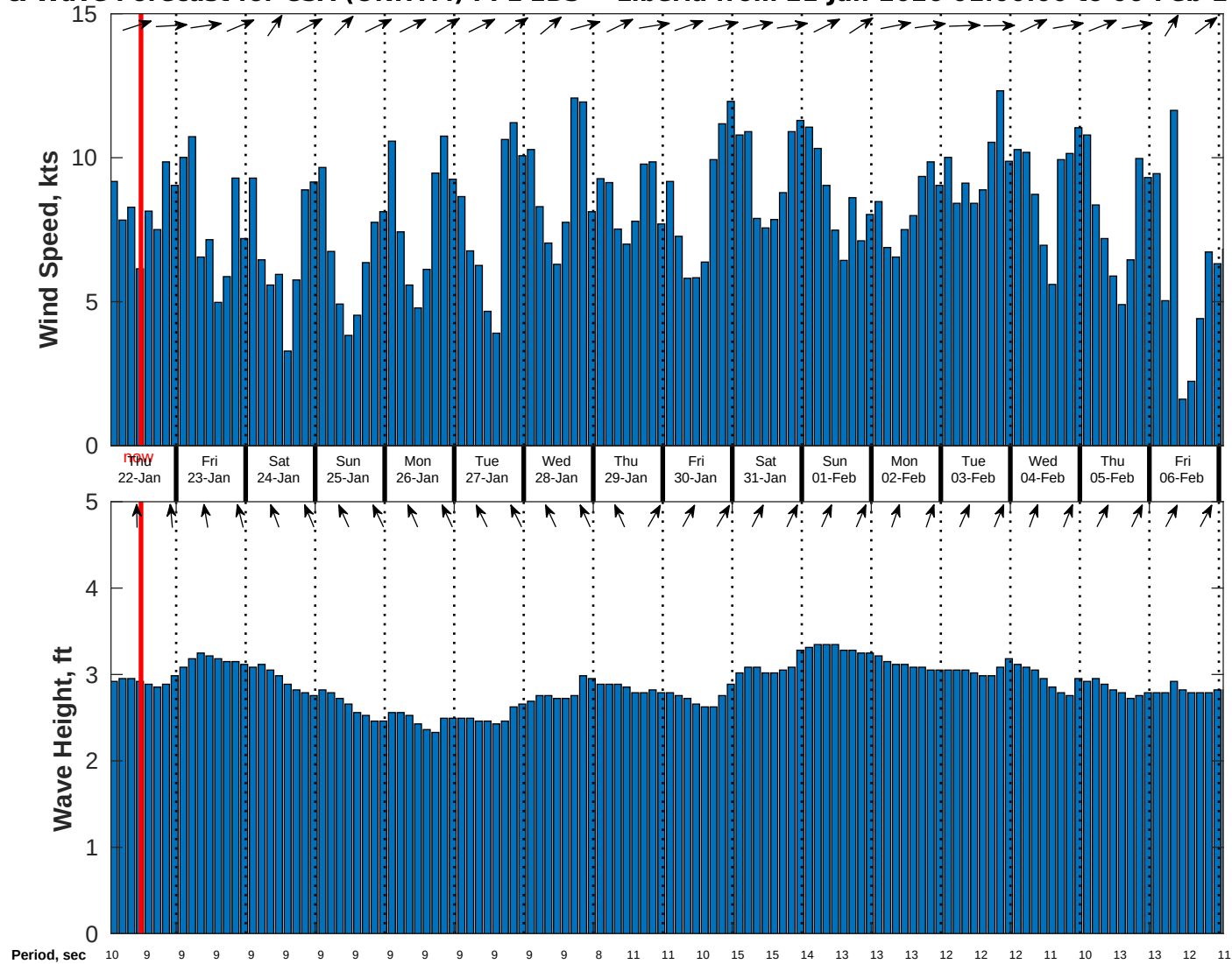
Wind & Wave Forecast for CSA (ONHYM) PPL EBS - Liberia from 21-Jan-2026 01:00:00 to 06-Feb-2026 01:00:00
