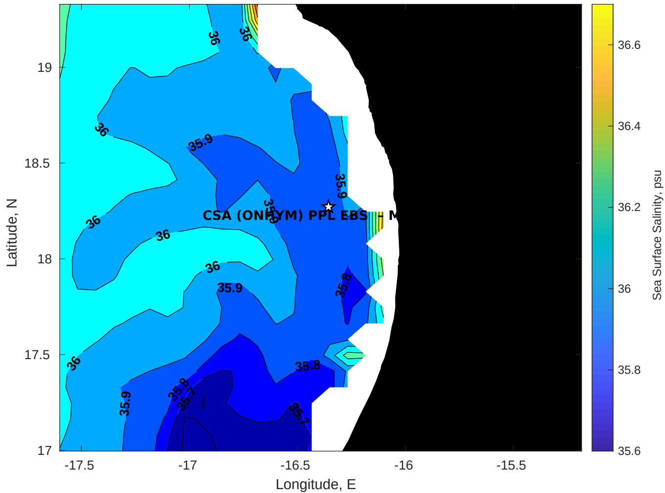
Surface Salinity for CSA (ONHYM) PPL EBS - Mauritania at 20-Jan-2026 00:00:00
