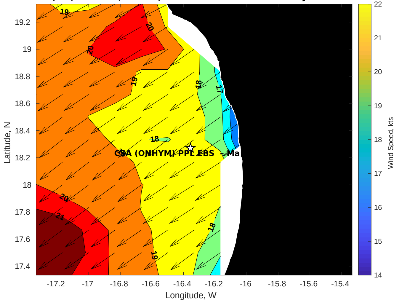
GFS Winds (kts) for CSA (ONHYM) PPL EBS - Mauritania at 21-Jan-2026 09:00:00
