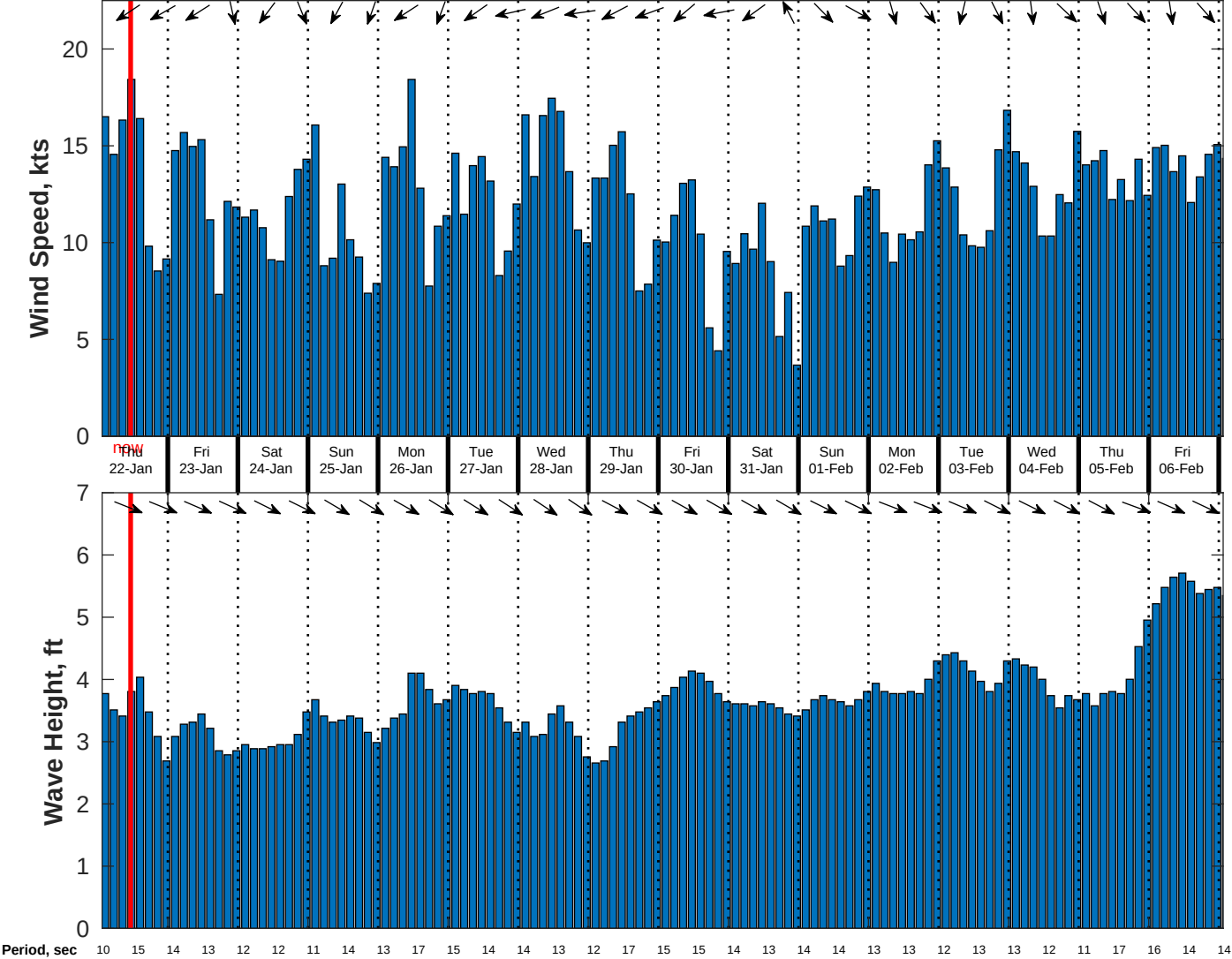
Wind & Wave Forecast for CSA (ONHYM) PPL EBS - Mauritania from 21-Jan-2026 01:00:00 to 06-Feb-2026 01:00:00
