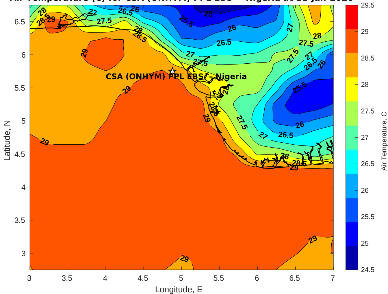
Air Temperature (C) for CSA (ONHYM) PPL EBS - Nigeria at 21-Jan-2026
