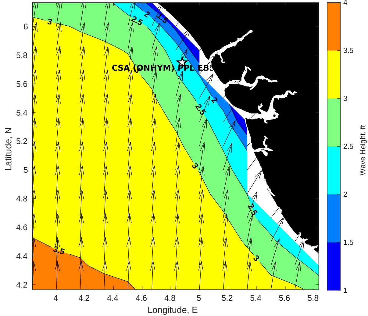
GFS Wave Height (ft) for CSA (ONHYM) PPL EBS - Nigeria at 21-Jan-2026 09:00:00
