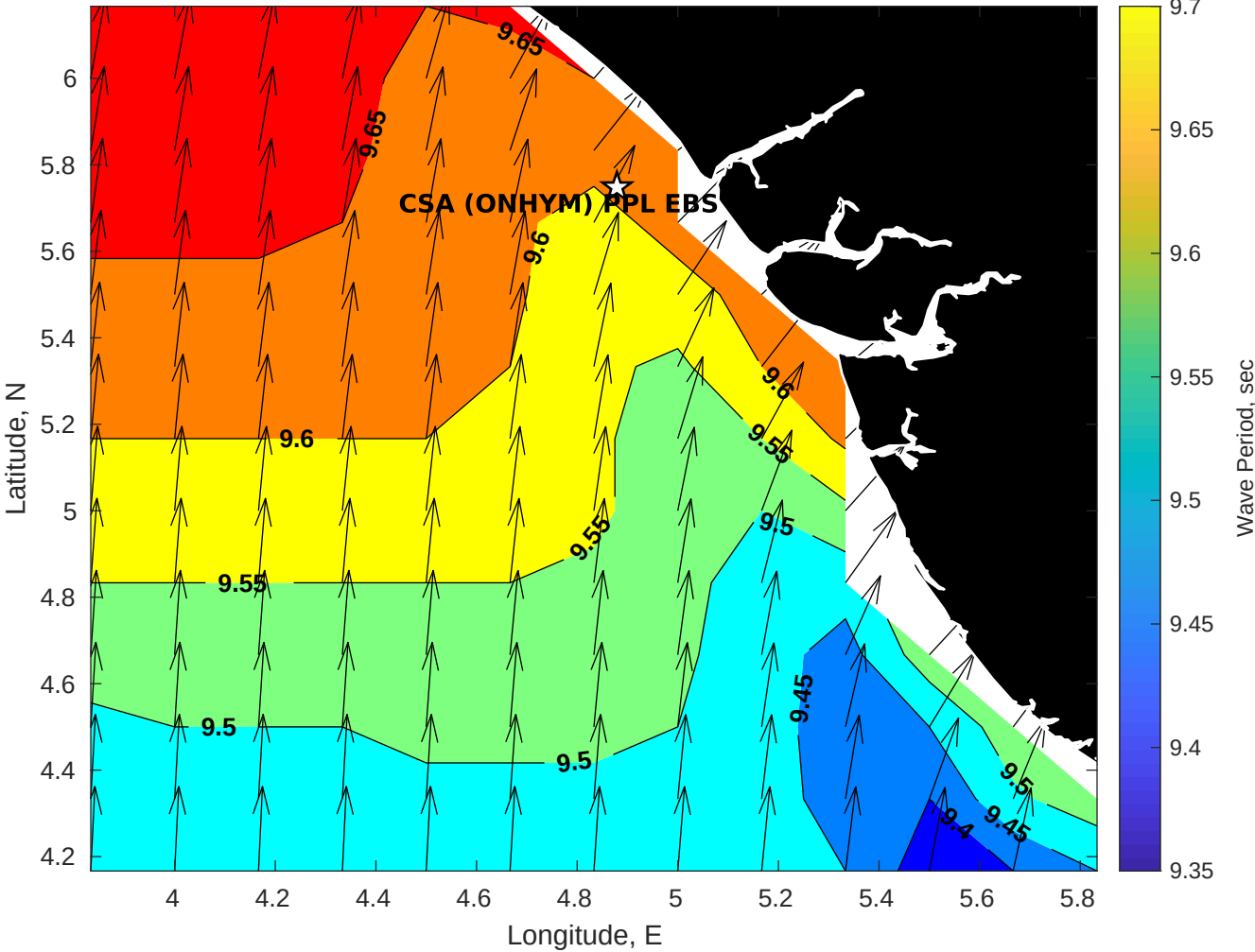
GFS Wave Period (sec) for CSA (ONHYM) PPL EBS - Nigeria at 21-Jan-2026 09:00:00
