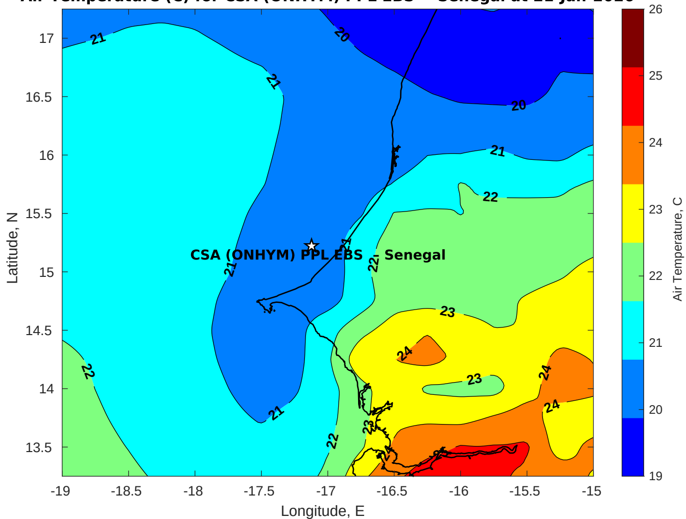
Air Temperature (C) for CSA (ONHYM) PPL EBS - Senegal at 21-Jan-2026
