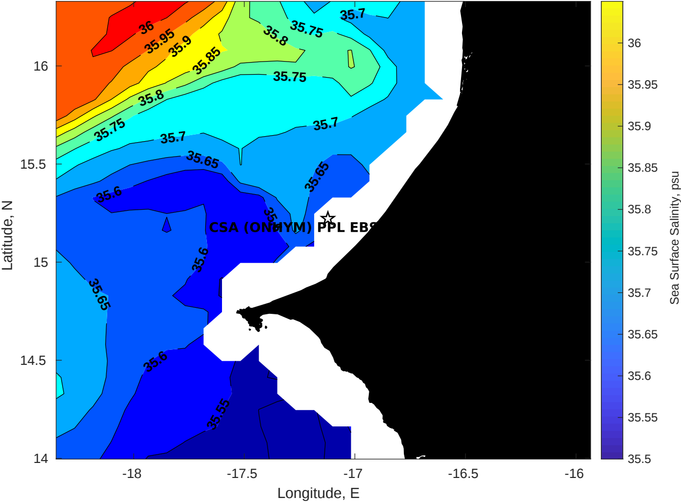
Surface Salinity for CSA (ONHYM) PPL EBS - Senegal at 20-Jan-2026 00:00:00
