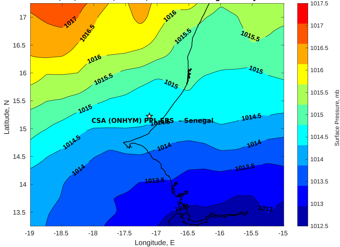
Surface Pressure (mb) for CSA (ONHYM) PPL EBS - Senegal at 21-Jan-2026 00:00:00
