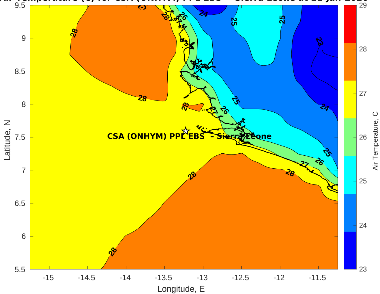
Air Temperature (C) for CSA (ONHYM) PPL EBS - Sierra Leone at 21-Jan-2026
