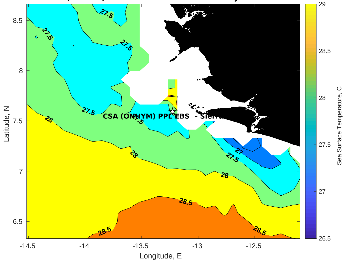
SST for CSA (ONHYM) PPL EBS - Sierra Leone at 20-Jan-2026 00:00:00
