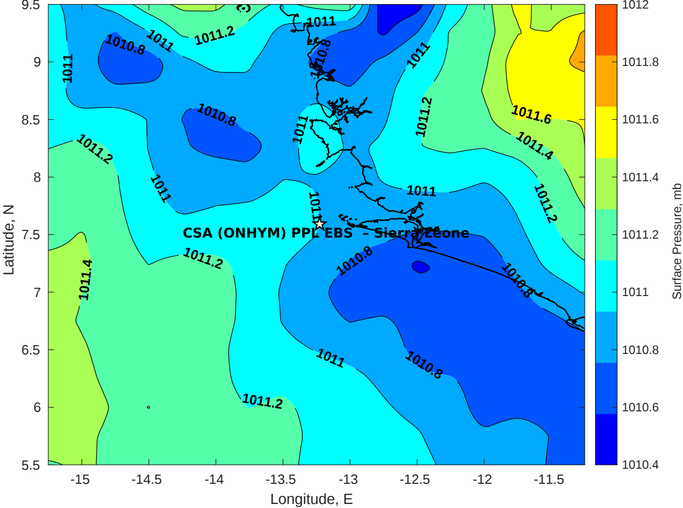
Surface Pressure (mb) for CSA (ONHYM) PPL EBS - Sierra Leone at 22-Jan-2026 00:00:00
