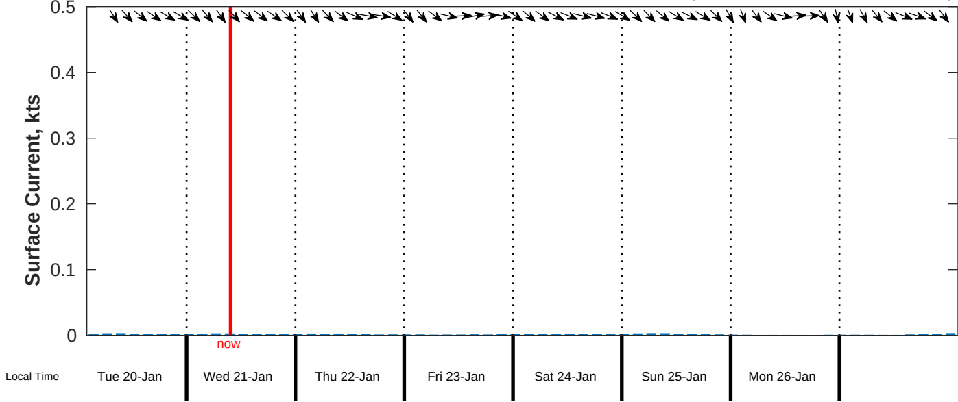
Surface Current Forecast for CSA (ONHYM) PPL EBS - Sierra Leone from 20-Jan-2026 00:00:00 to 28-Jan-2026 00:00:00
