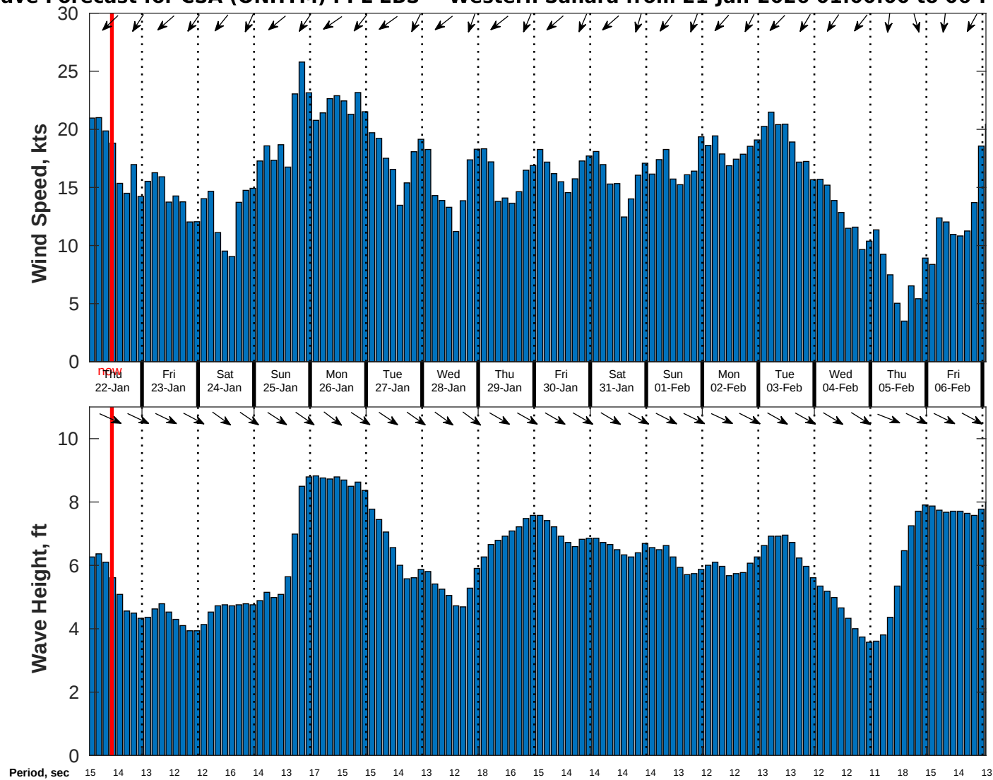
Wind & Wave Forecast for CSA (ONHYM) PPL EBS - Western Sahara from 21-Jan-2026 01:00:00 to 06-Feb-2026 01:00:00
