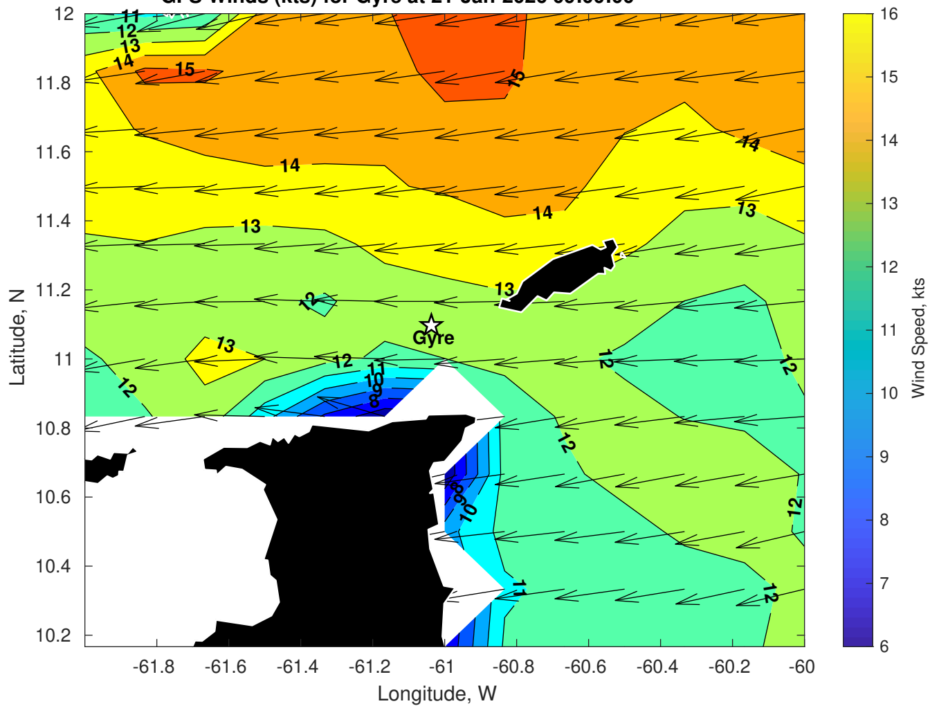
GFS Winds (kts) for Gyre at 21-Jan-2026 09:00:00
