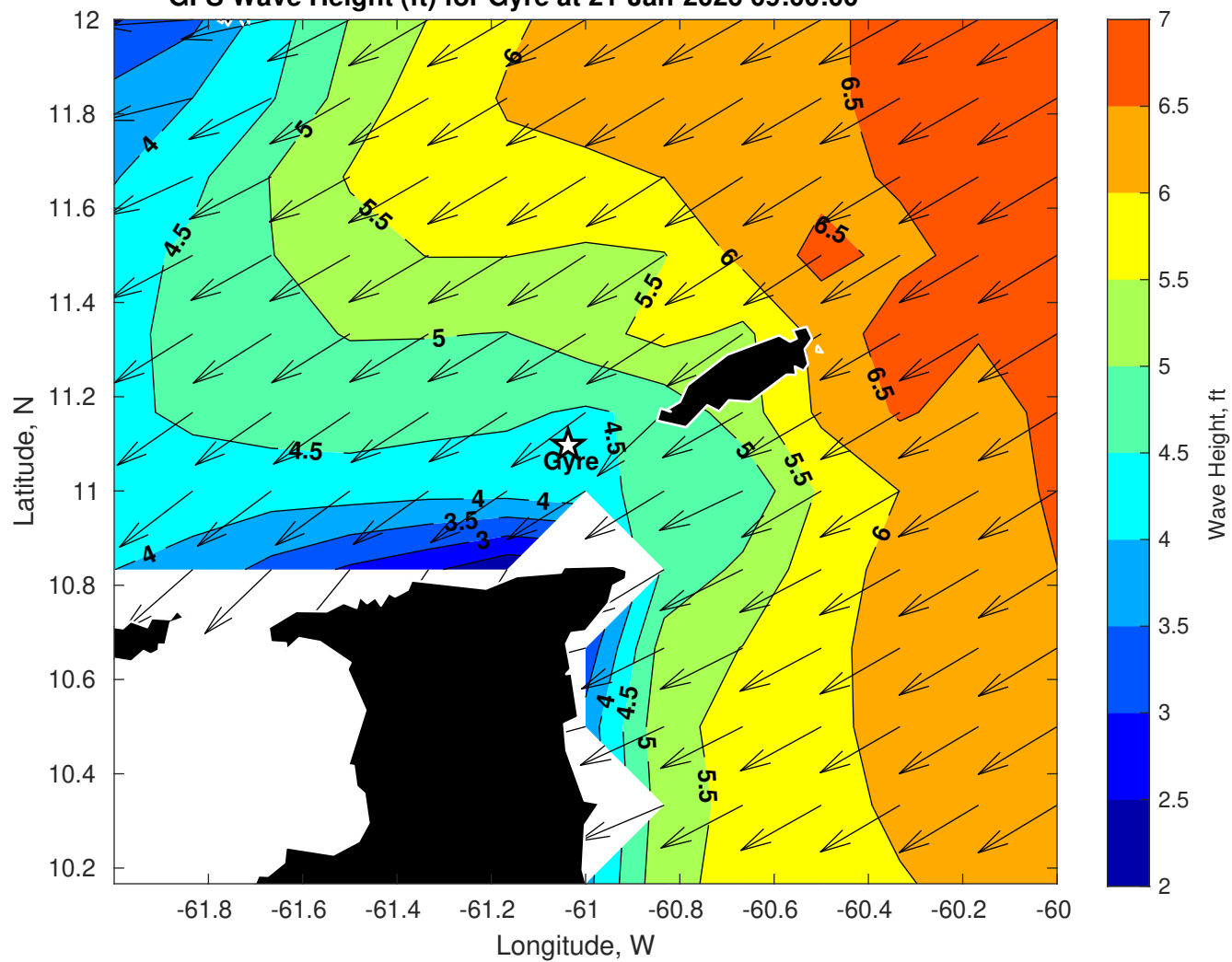
GFS Wave Height (ft) for Gyre at 21-Jan-2026 09:00:00
