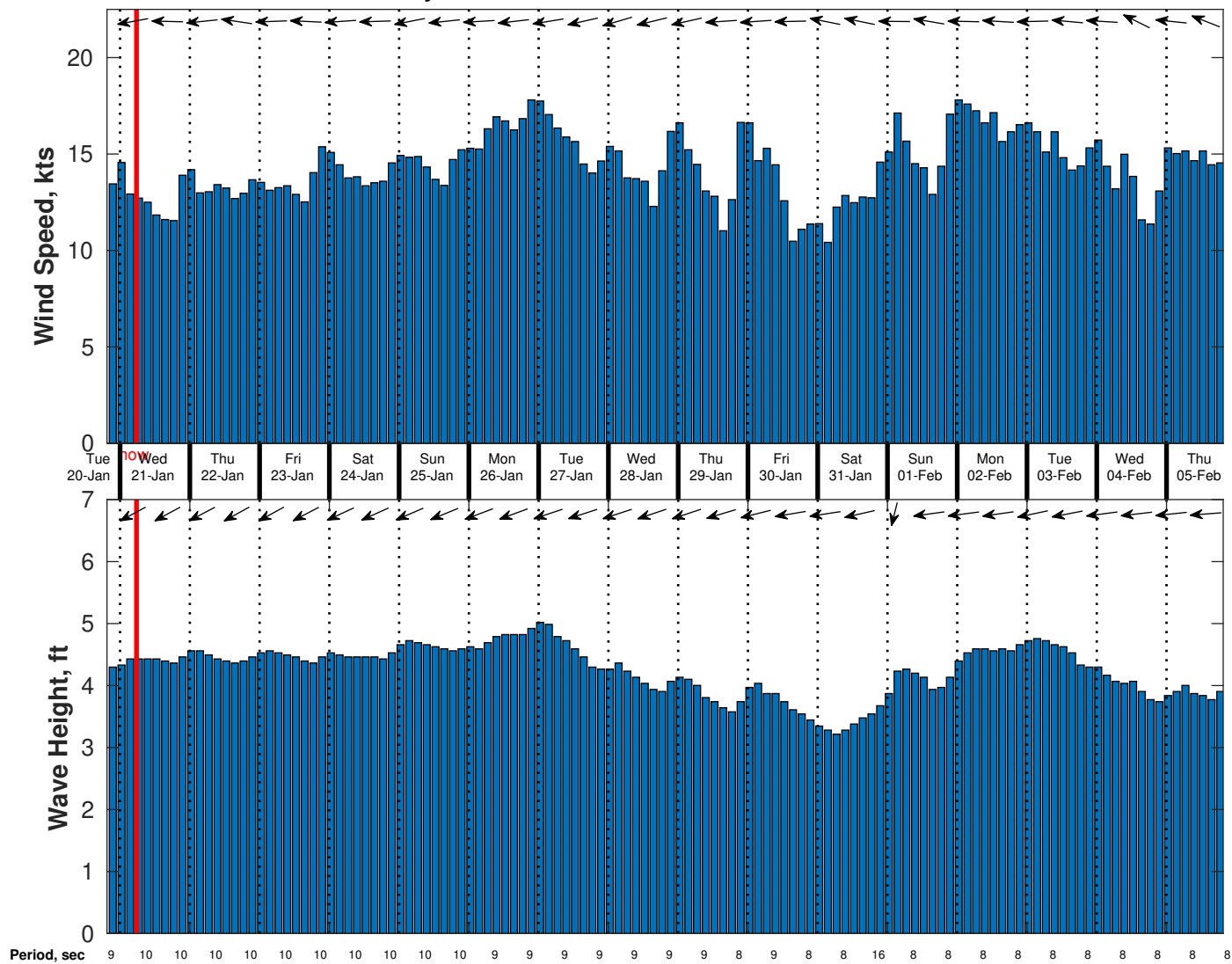
Wind & Wave Forecast for Gyre from 20-Jan-2026 20:00:00 to 05-Feb-2026 20:00:00
