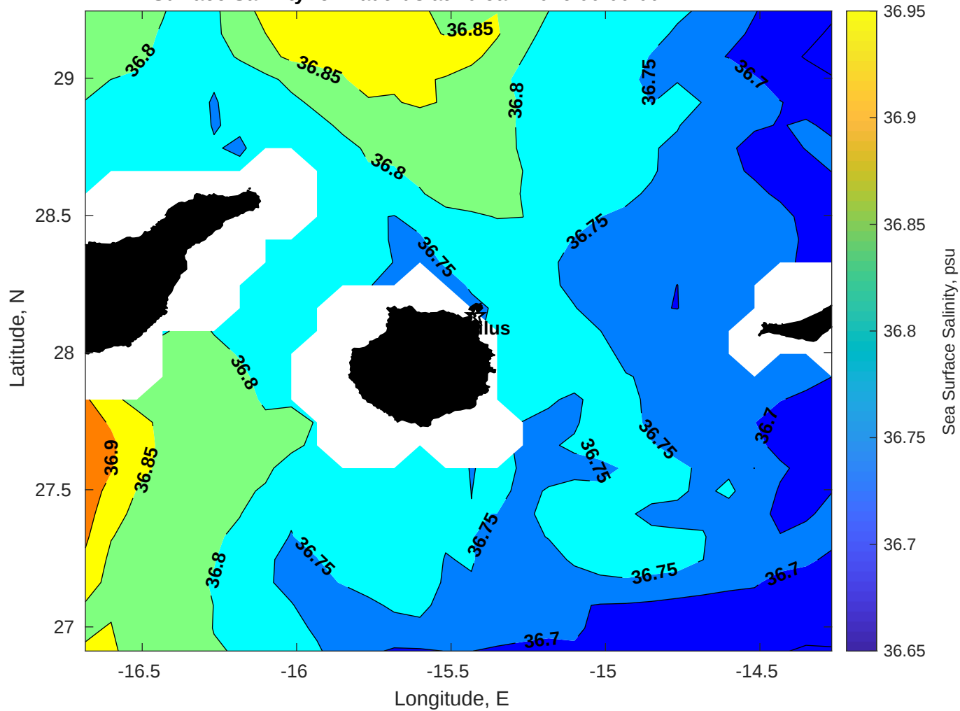
Surface Salinity for Nautilus at 20-Jan-2026 00:00:00
