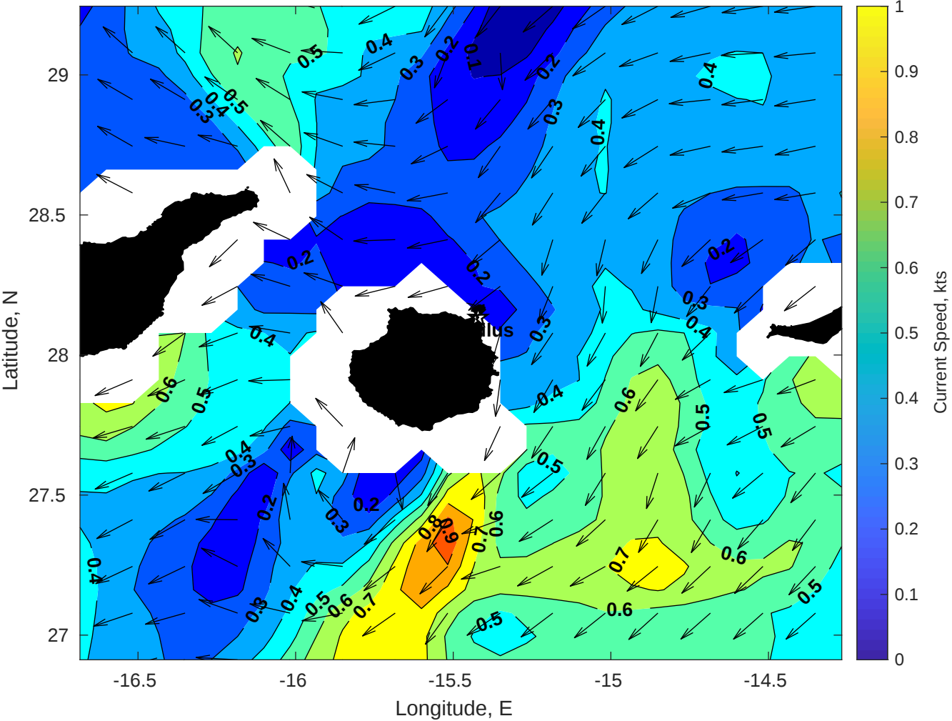
Surface Currents for Nautilus at 20-Jan-2026 00:00:00
