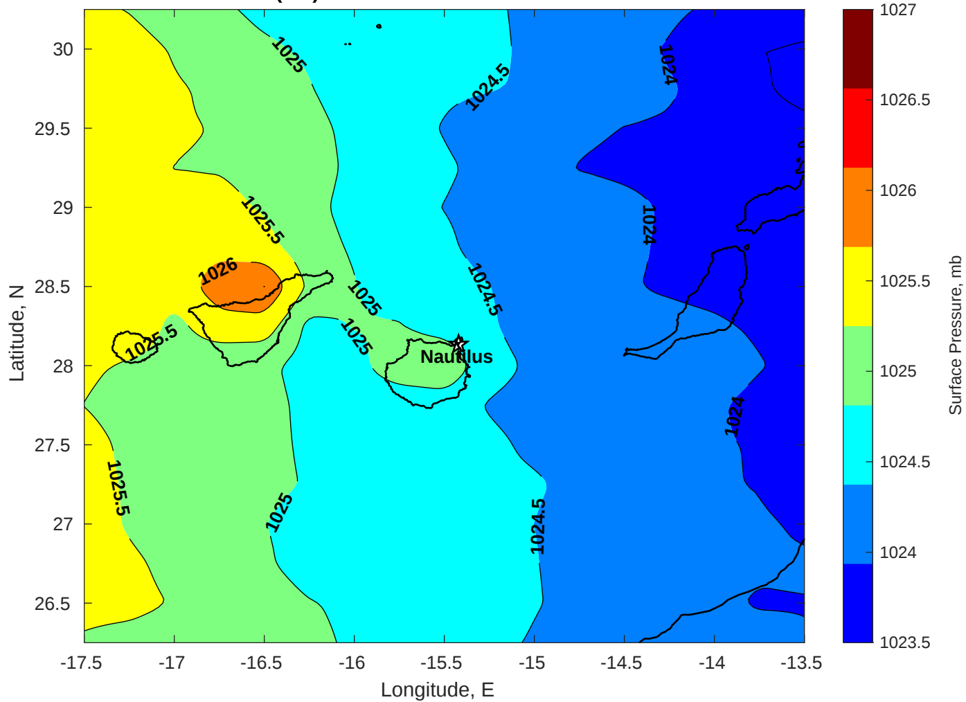
Surface Pressure (mb) for Nautilus at 21-Jan-2026 00:00:00
