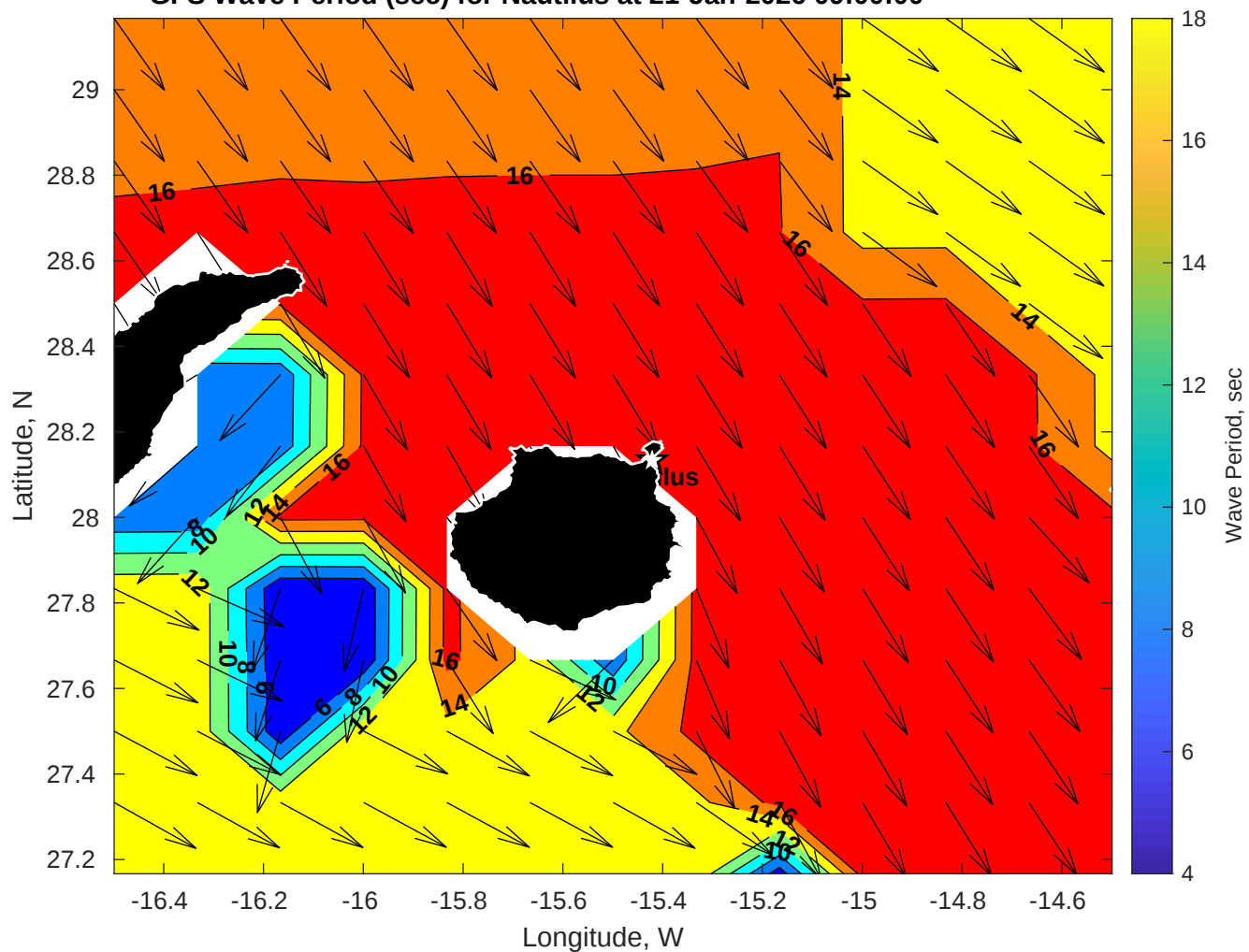
GFS Wave Period (sec) for Nautilus at 21-Jan-2026 09:00:00
