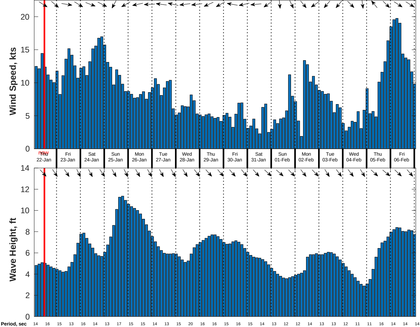
Wind & Wave Forecast for Nautilus from 21-Jan-2026 02:00:00 to 06-Feb-2026 02:00:00
