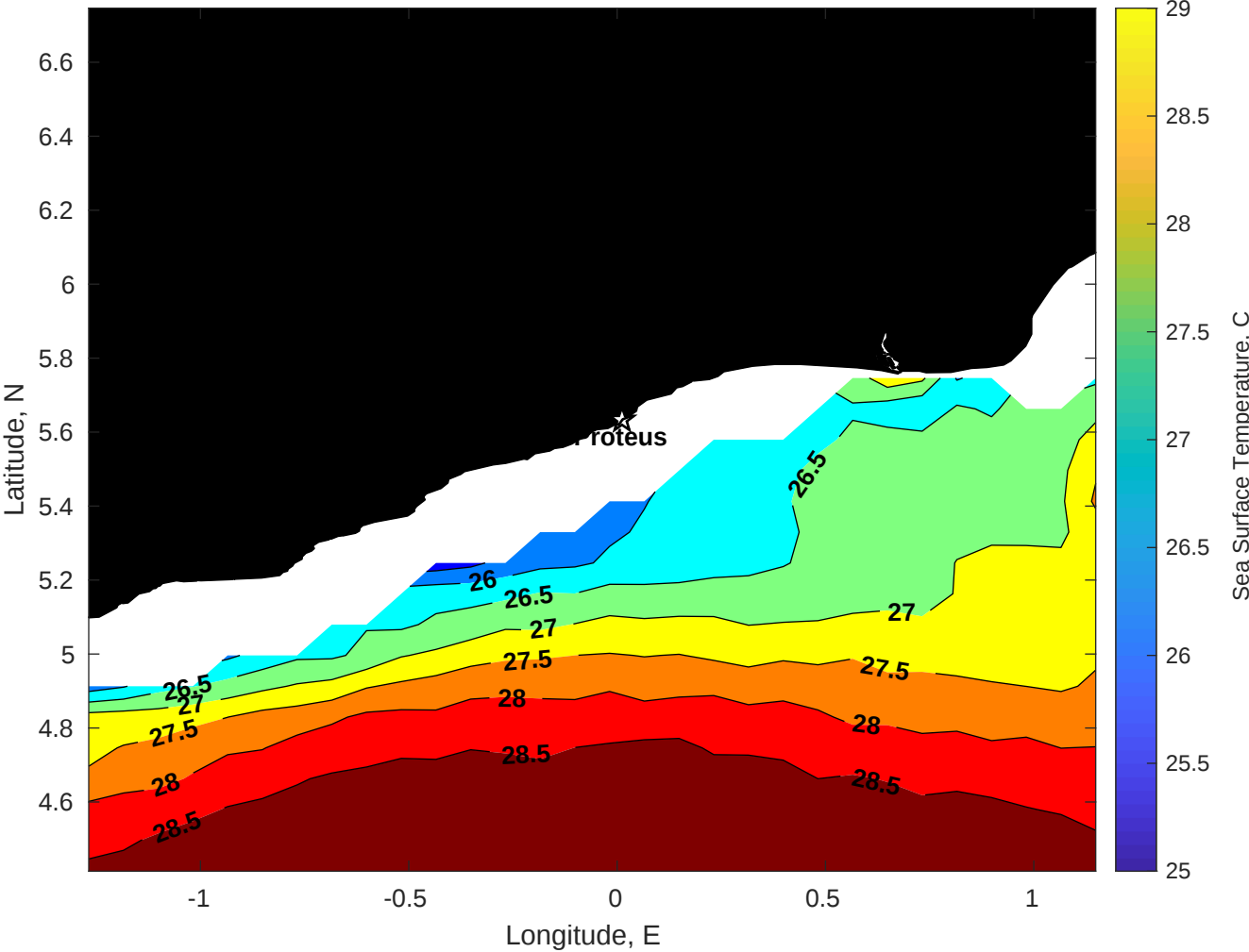
SST for Proteus at 20-Jan-2026 00:00:00
