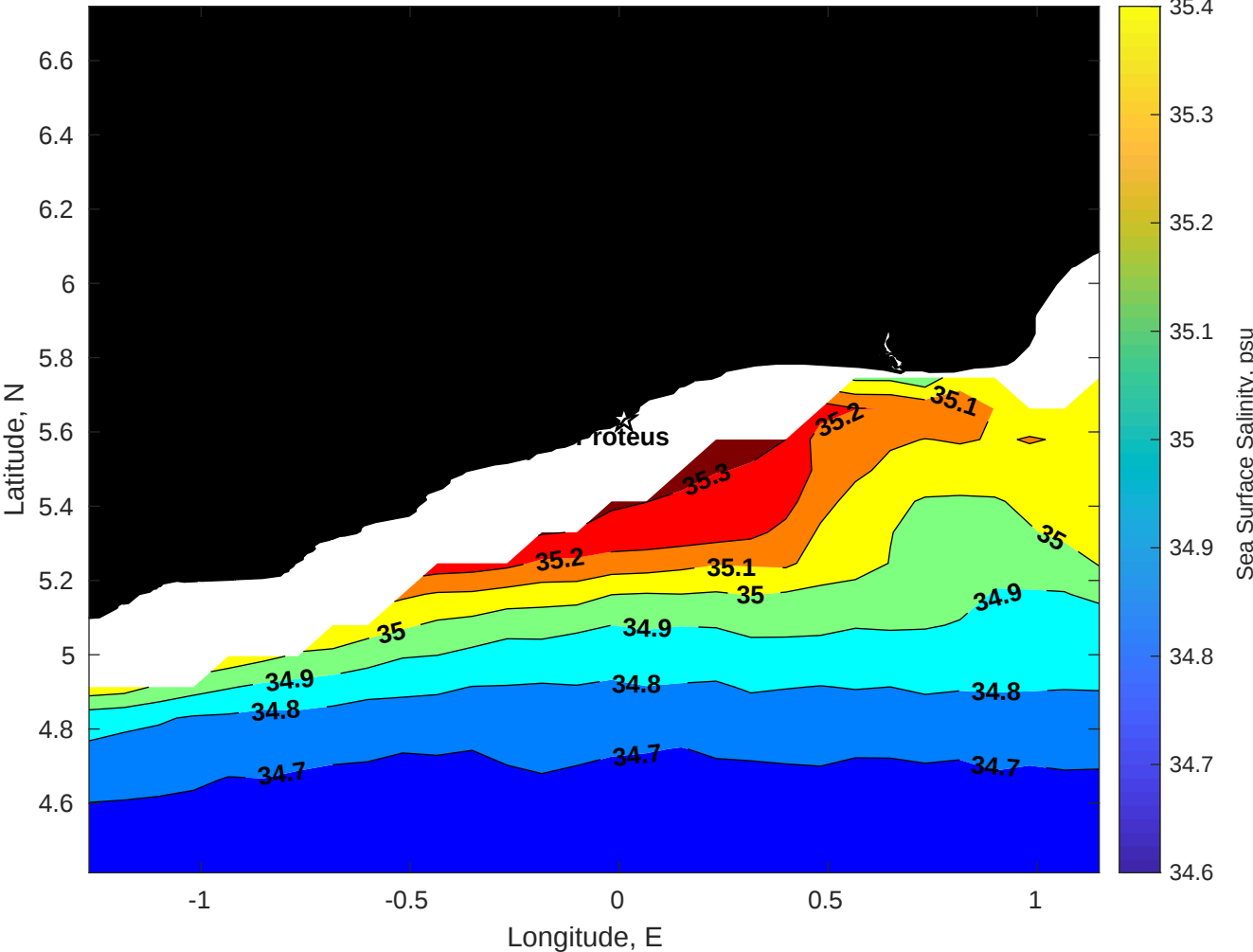
Surface Salinity for Proteus at 20-Jan-2026 00:00:00
