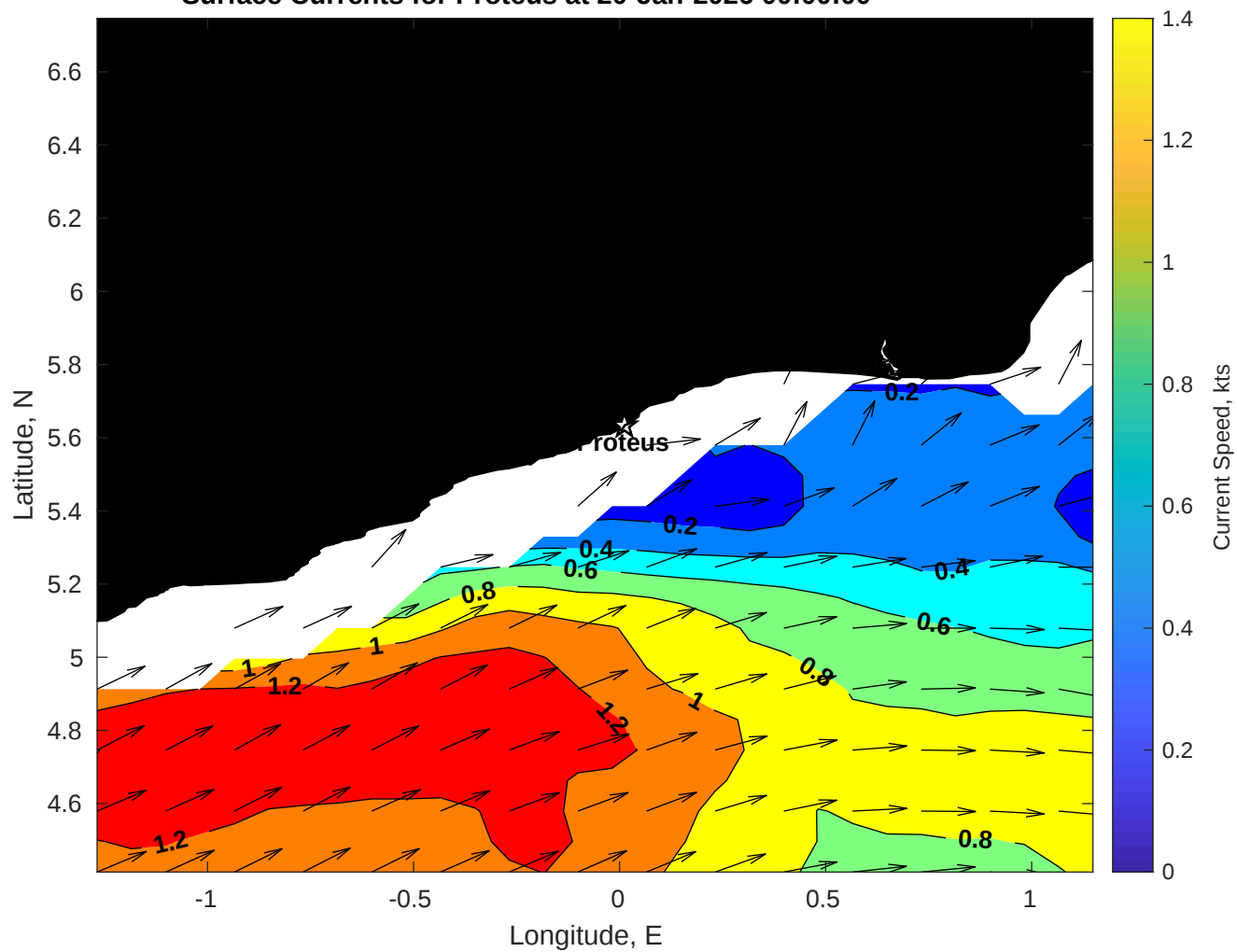
Surface Currents for Proteus at 20-Jan-2026 00:00:00
