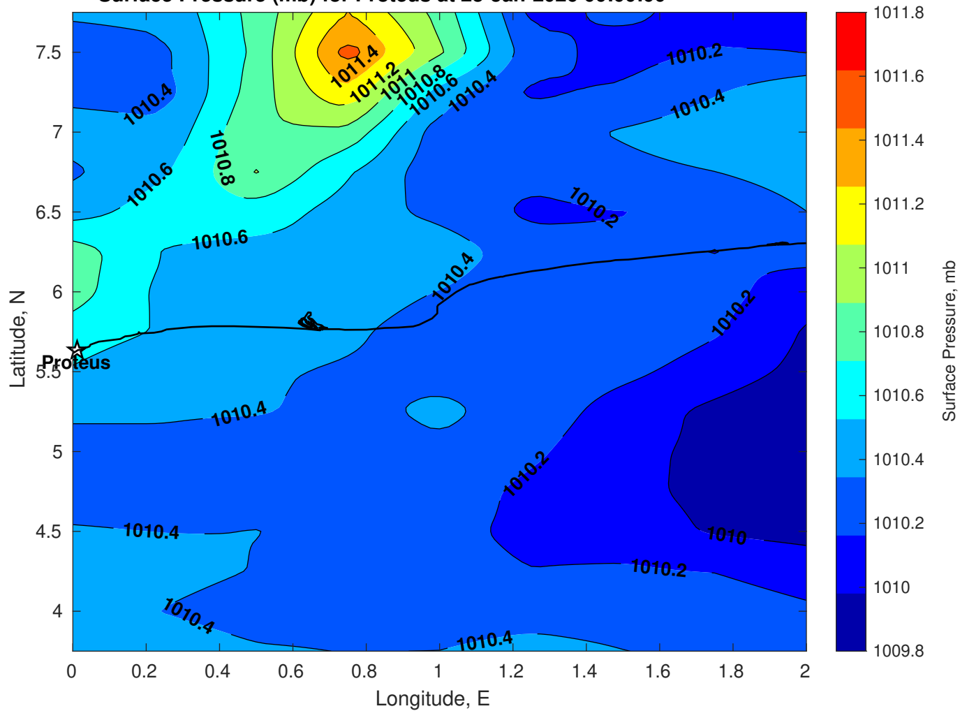
Surface Pressure (mb) for Proteus at 23-Jan-2026 00:00:00
