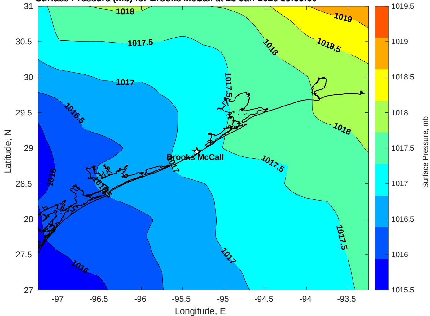
Surface Pressure (mb) for Brooks McCall at 23-Jan-2026 00:00:00
