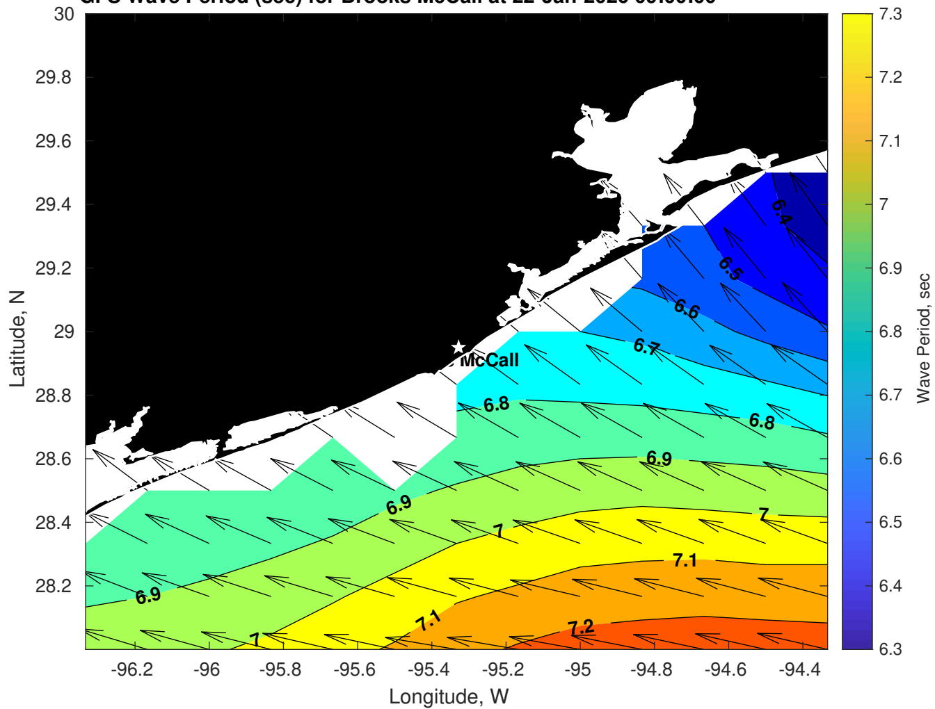
GFS Wave Period (sec) for Brooks McCall at 22-Jan-2026 09:00:00
