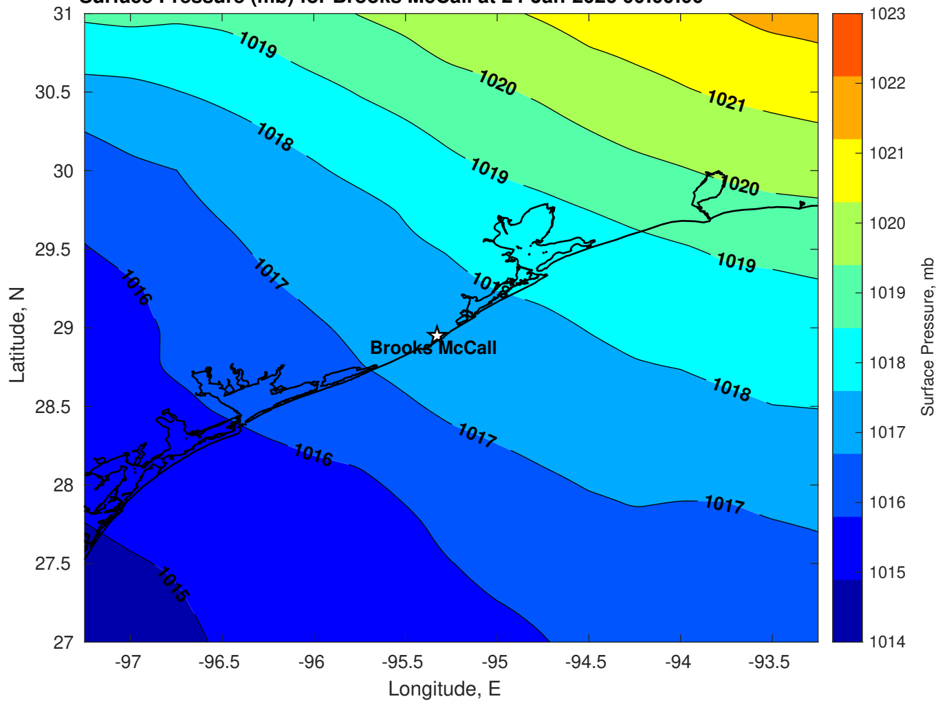
Surface Pressure (mb) for Brooks McCall at 24-Jan-2026 00:00:00
