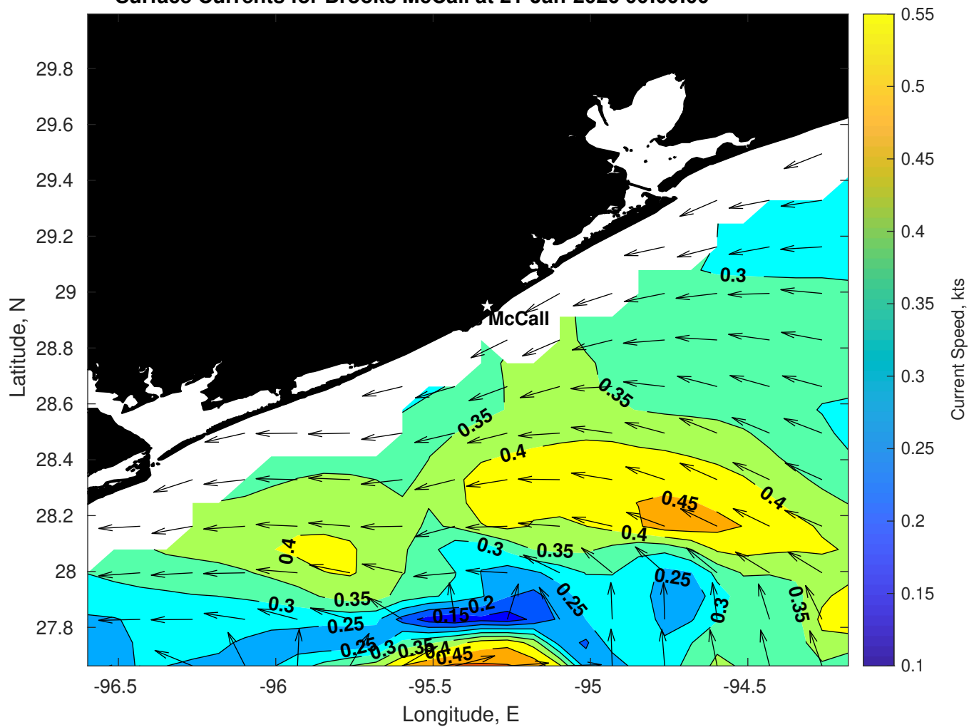
Surface Currents for Brooks McCall at 21-Jan-2026 00:00:00
