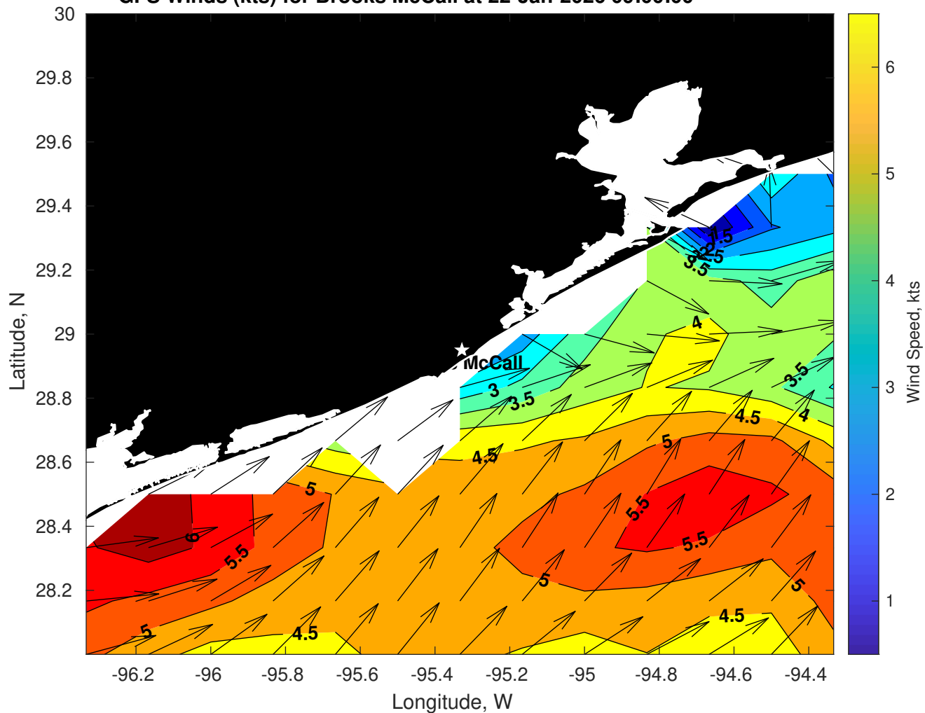
GFS Winds (kts) for Brooks McCall at 22-Jan-2026 09:00:00
