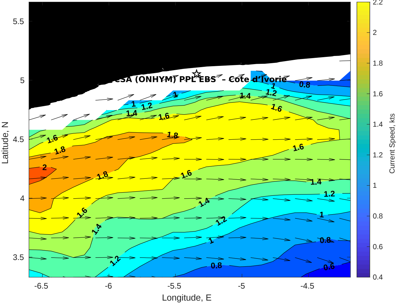
Surface Currents for CSA (ONHYM) PPL EBS - Cote d'Ivoire at 21-Jan-2026 00:00:00
