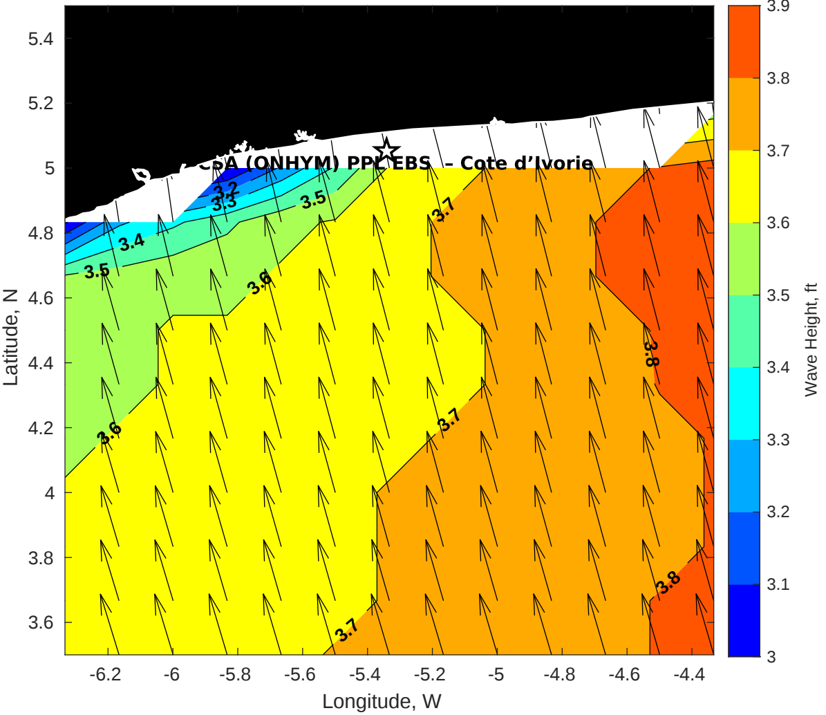
GFS Wave Height (ft) for CSA (ONHYM) PPL EBS - Cote d'Ivoire at 22-Jan-2026 09:00:00
