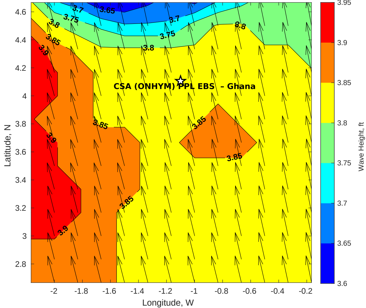
GFS Wave Height (ft) for CSA (ONHYM) PPL EBS - Ghana at 22-Jan-2026 09:00:00
