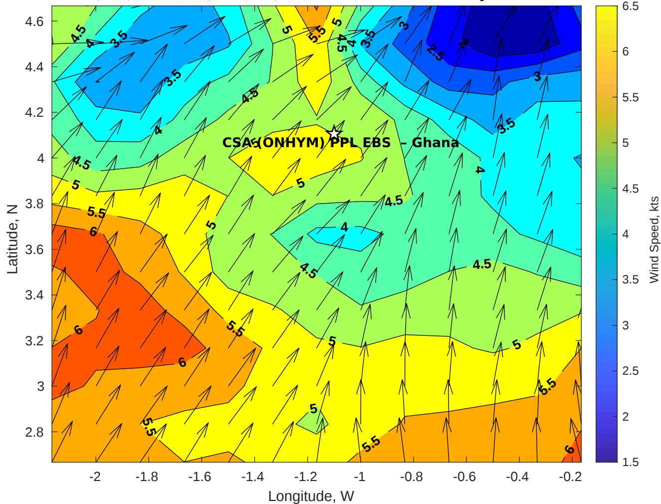
GFS Winds (kts) for CSA (ONHYM) PPL EBS - Ghana at 22-Jan-2026 09:00:00
