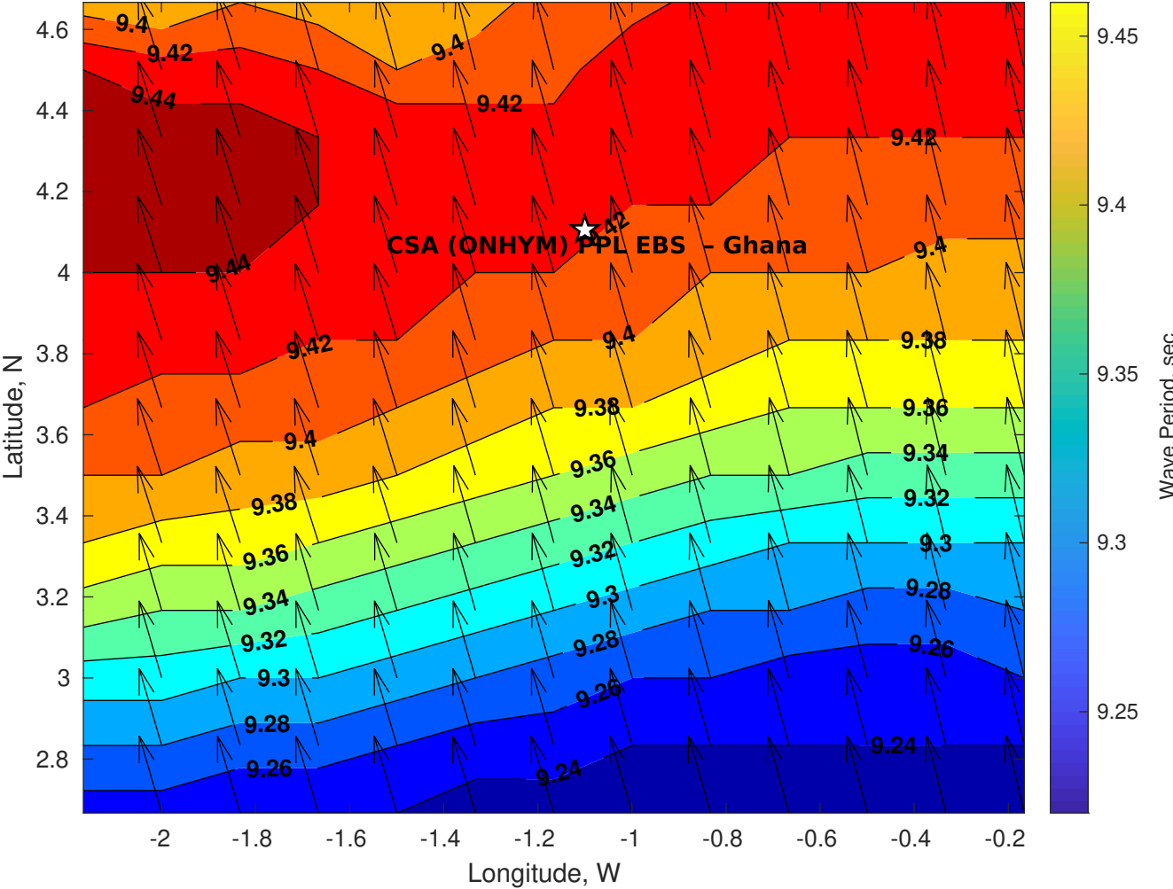
GFS Wave Period (sec) for CSA (ONHYM) PPL EBS - Ghana at 22-Jan-2026 09:00:00
