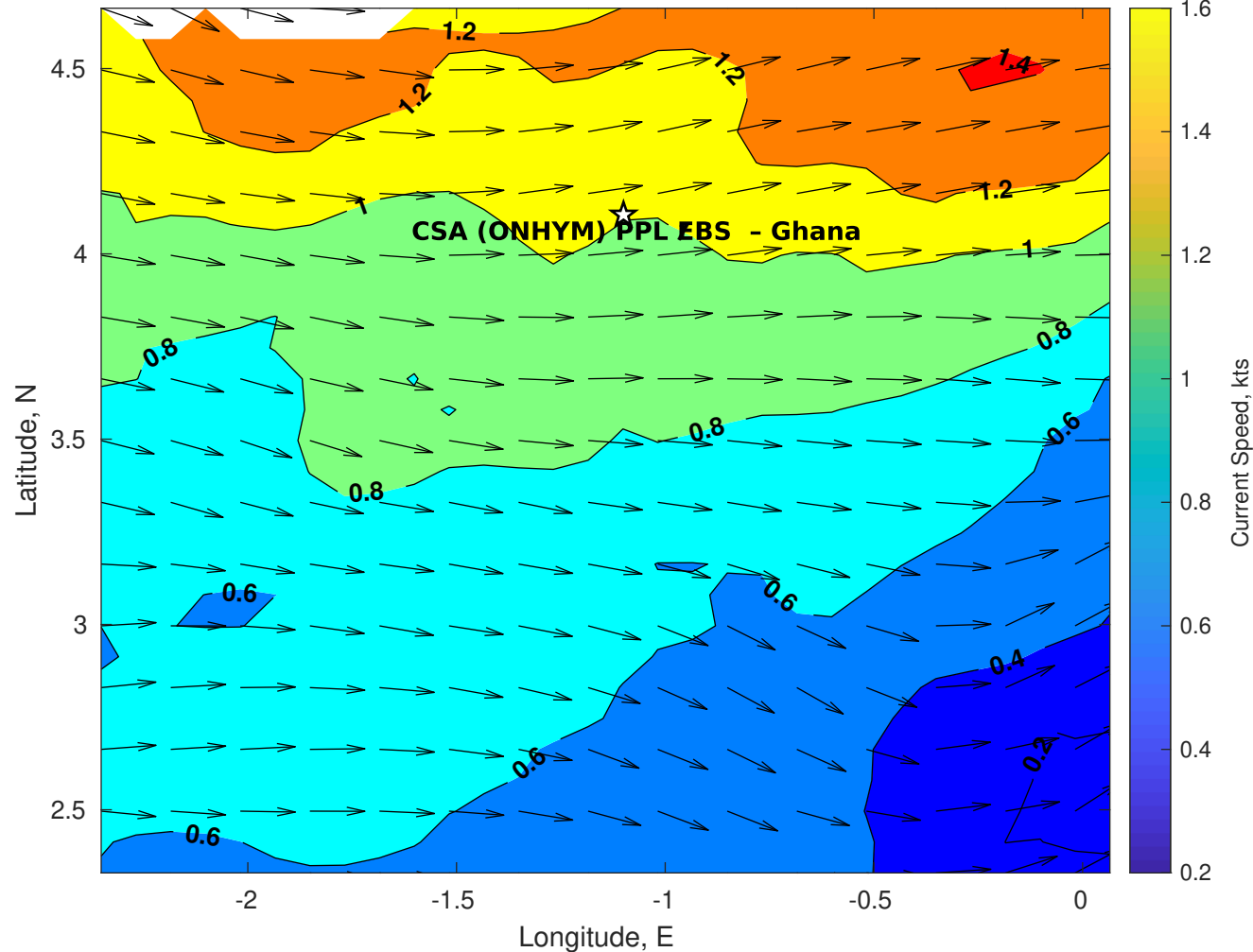
Surface Currents for CSA (ONHYM) PPL EBS - Ghana at 21-Jan-2026 00:00:00
